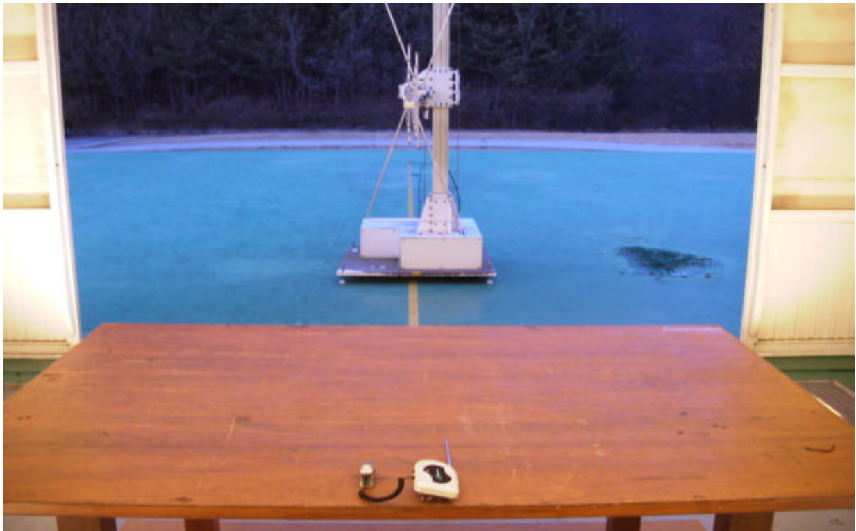
Radiated Emissions (fully extended antenna)
