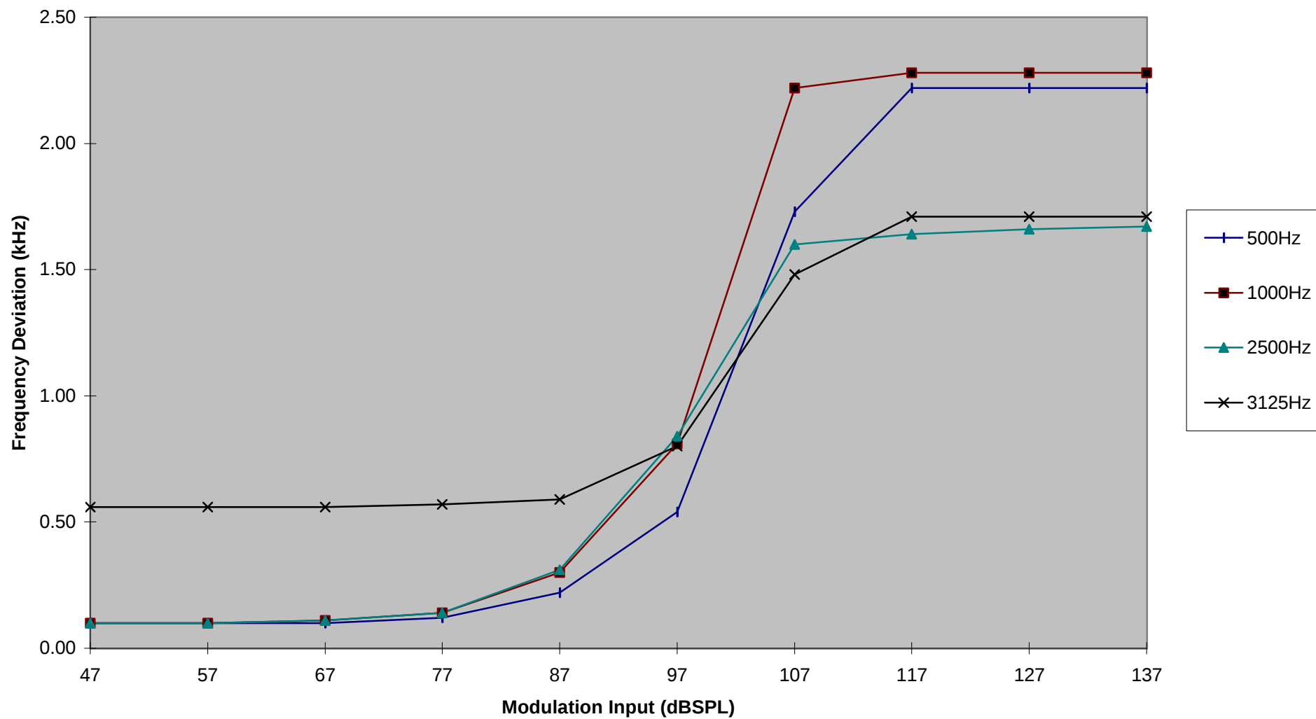
Modulation Limiting Characteristic (Model: YURI-01)
