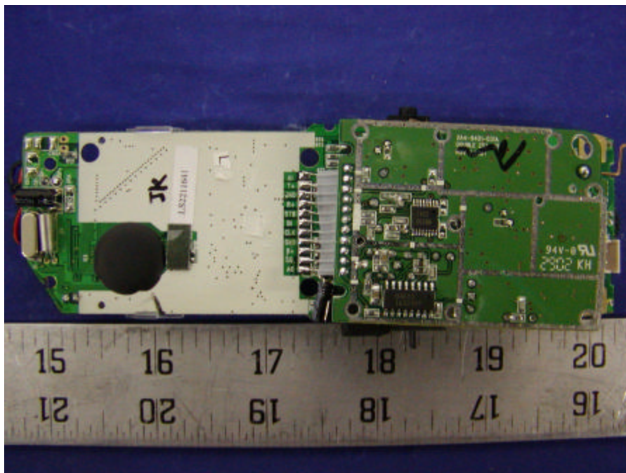
Handset - Component View 2
