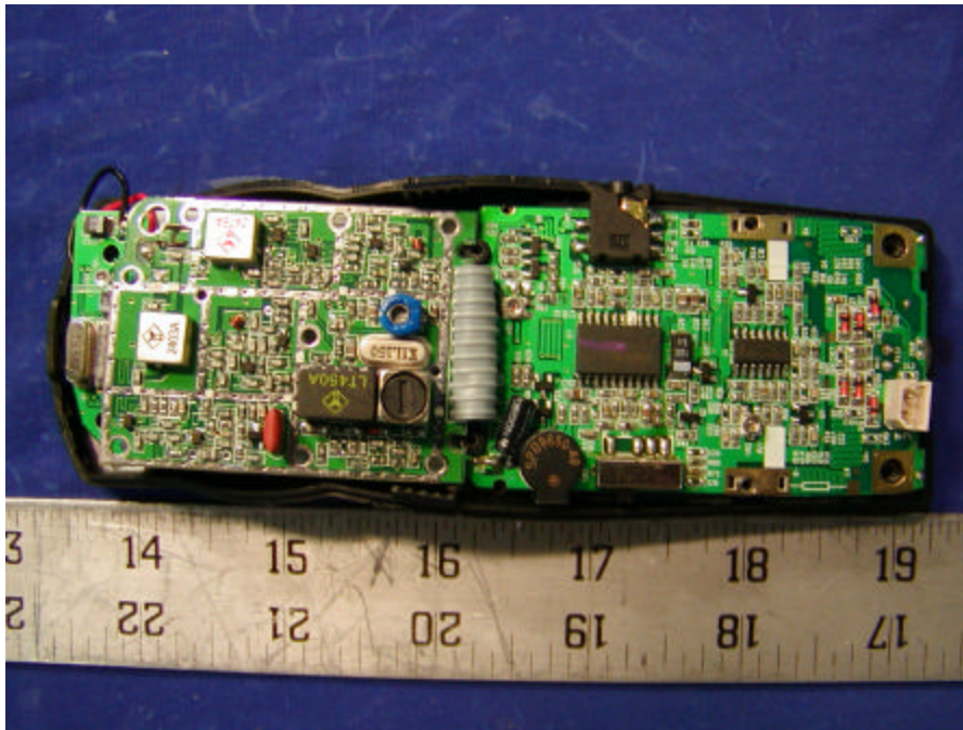
Handset - Component View 1
