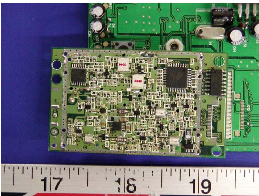
EUT – Daughter Board Bottom Shield Cover off Component View
