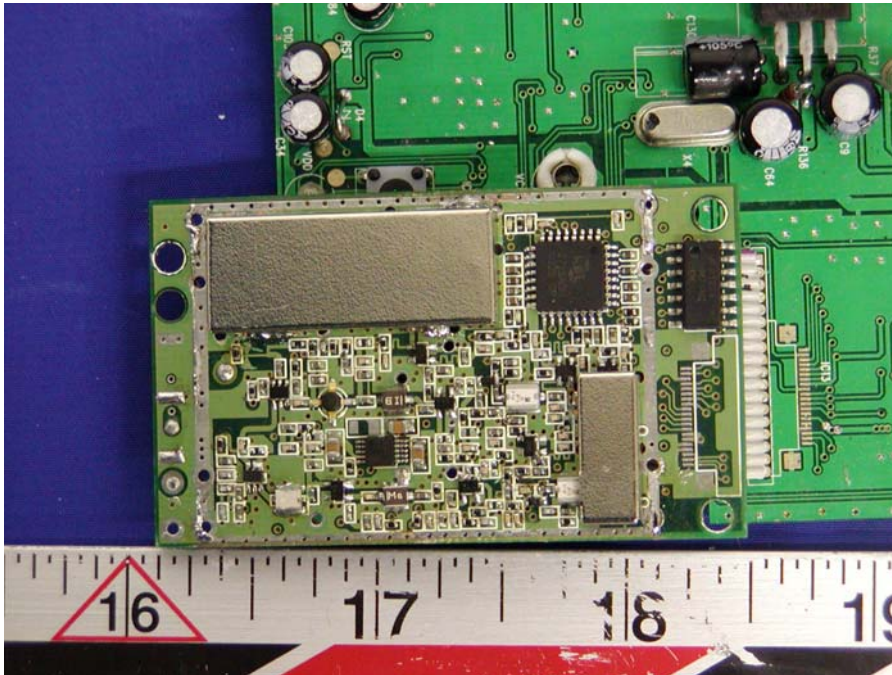
EUT – Daughter Board Top Shield Cover off Component View
