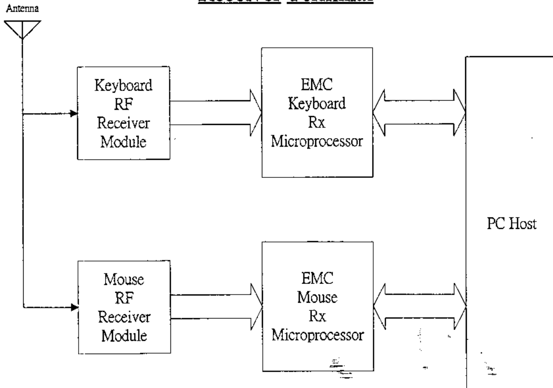
Fig.3 Receiver Block
