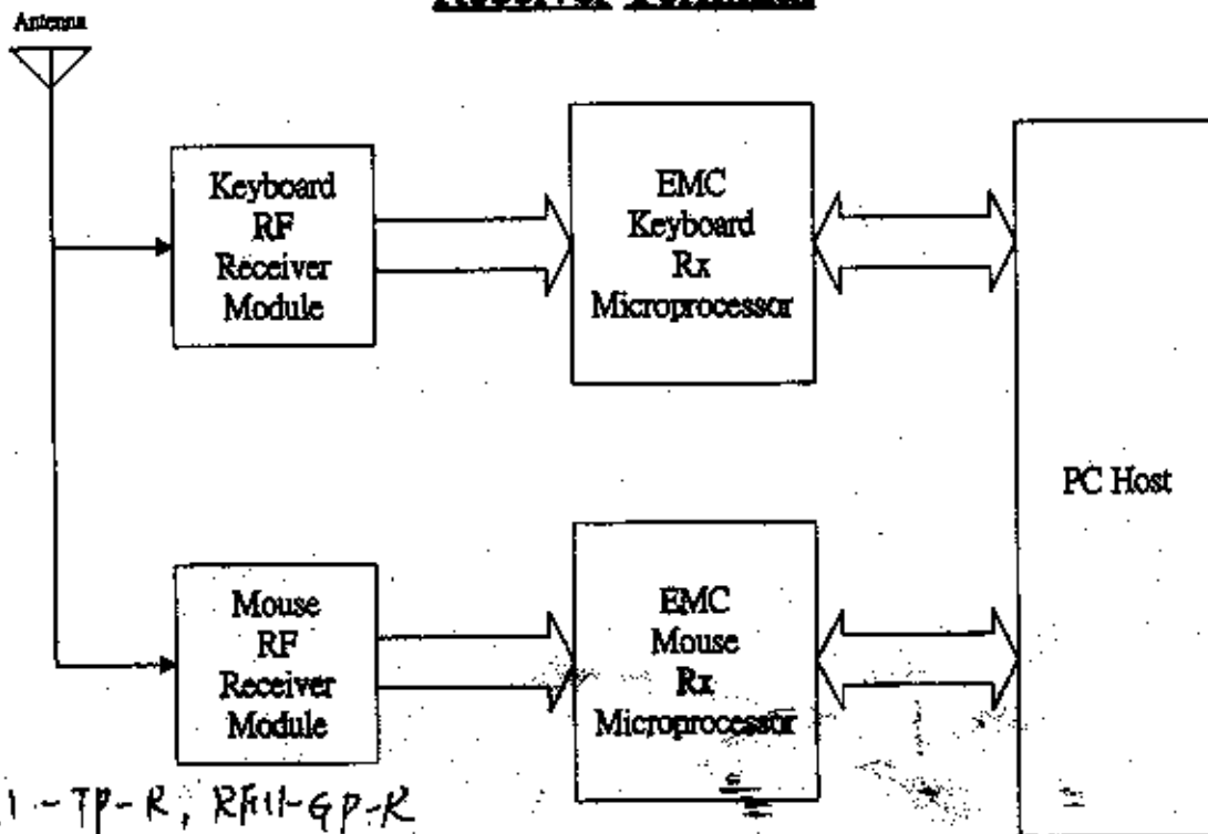
Fig.3 Receiver Block
