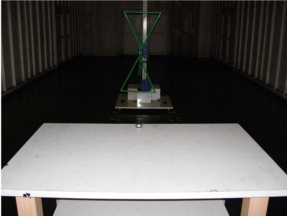
Back View of Radiated Test (M/N:26-284)
