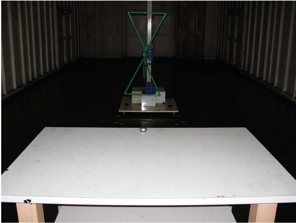
Back View of Radiated Test - (M/N:N530,N332)
