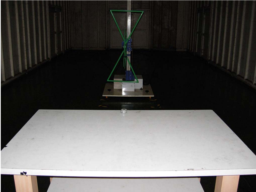
Back View of Radiated Test-(M/N: M310)
