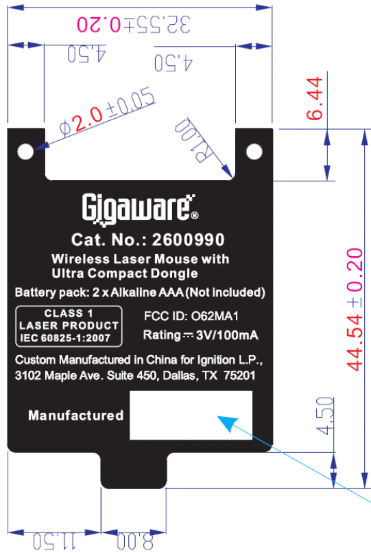
FCC ID Label Location
