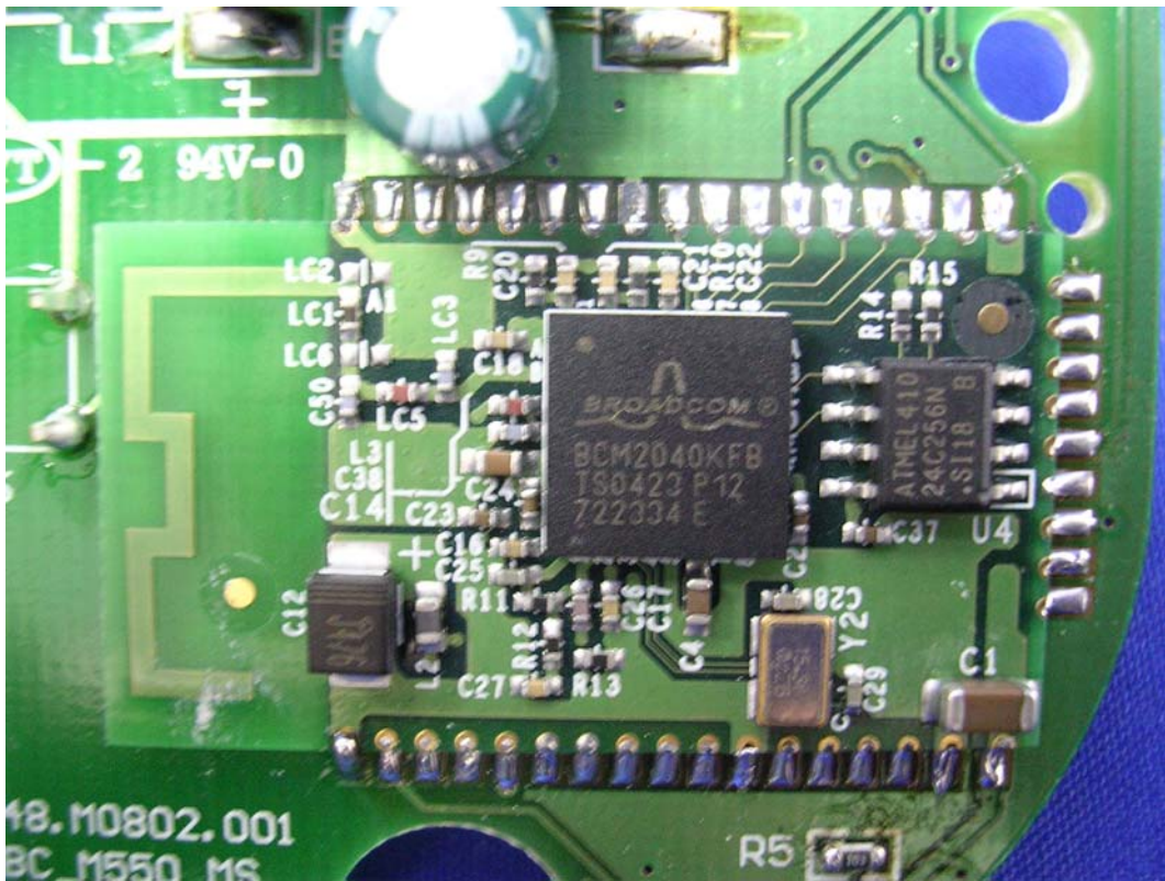
(7) EUT Photo
