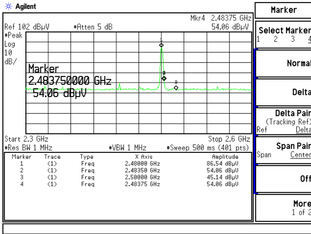
Figure Channel 78: (Horizontal)
