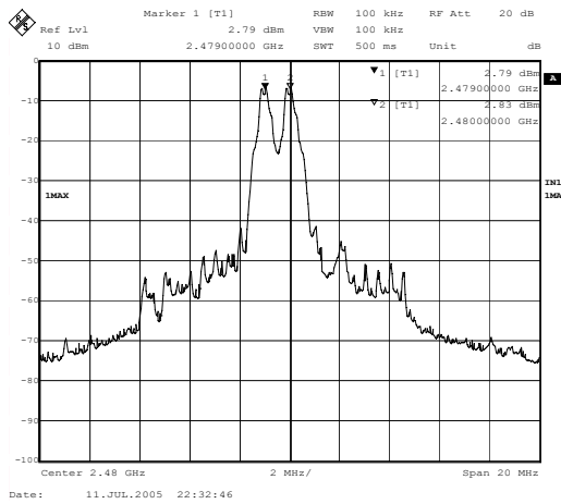
Channel 78 2480 MHz
