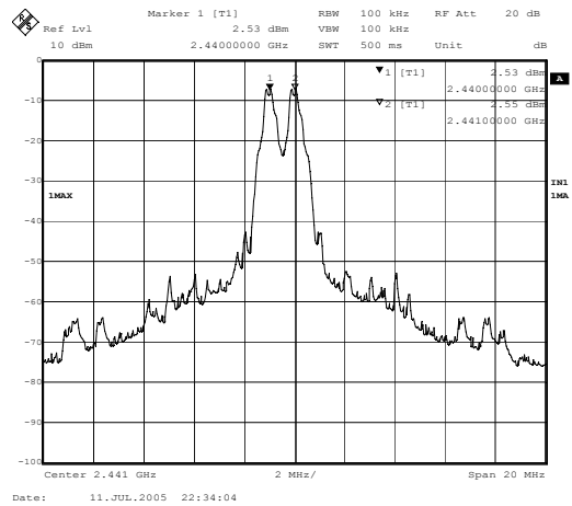
Channel 39 2441MHz
