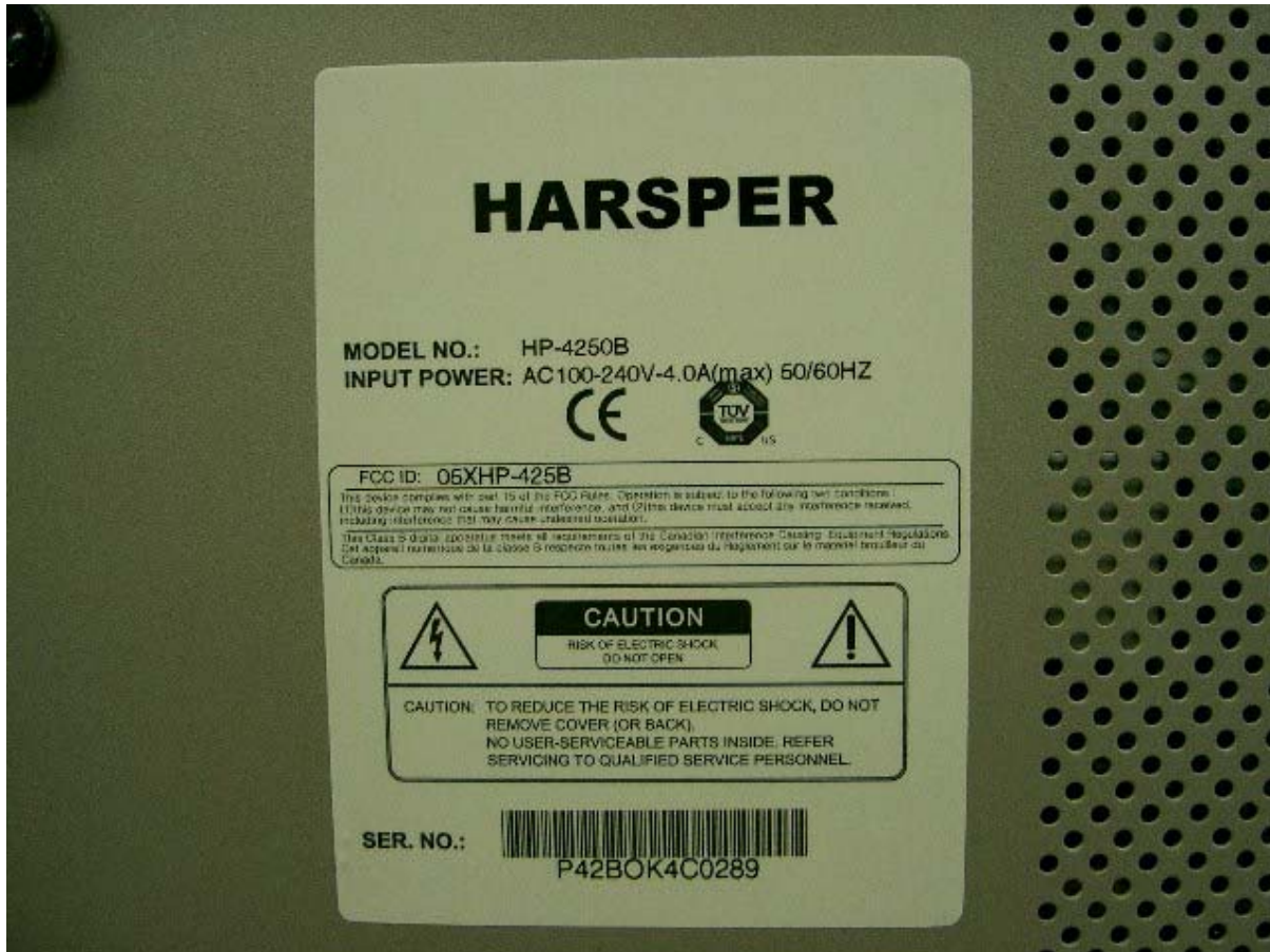
Figure 3.1 PRODUCT LABEL
