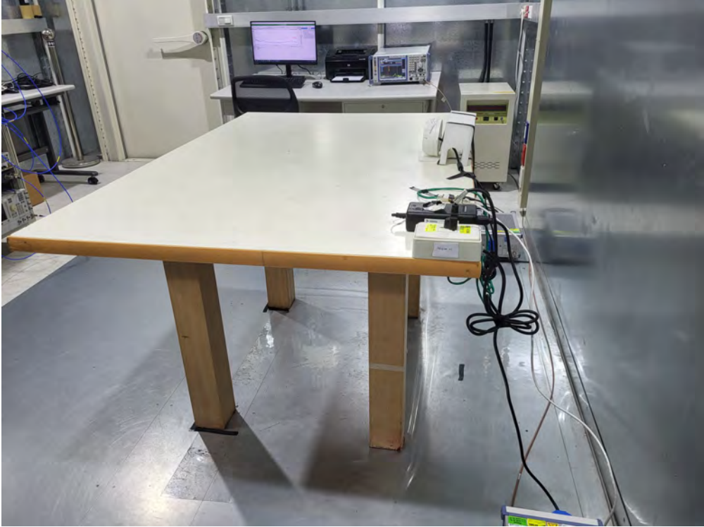
Conducted Test
