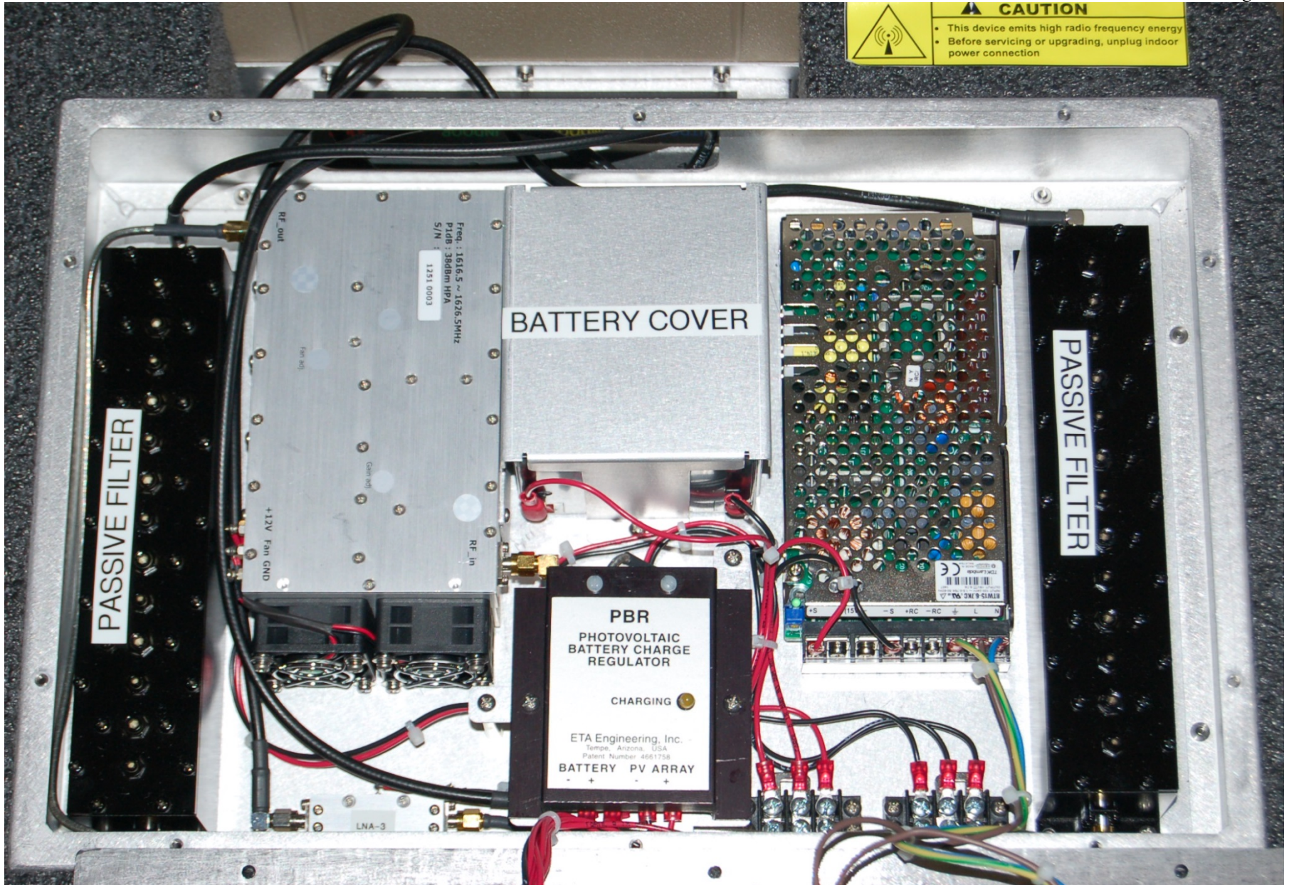
Figure 4 - Internal View - Main Items Labeled
