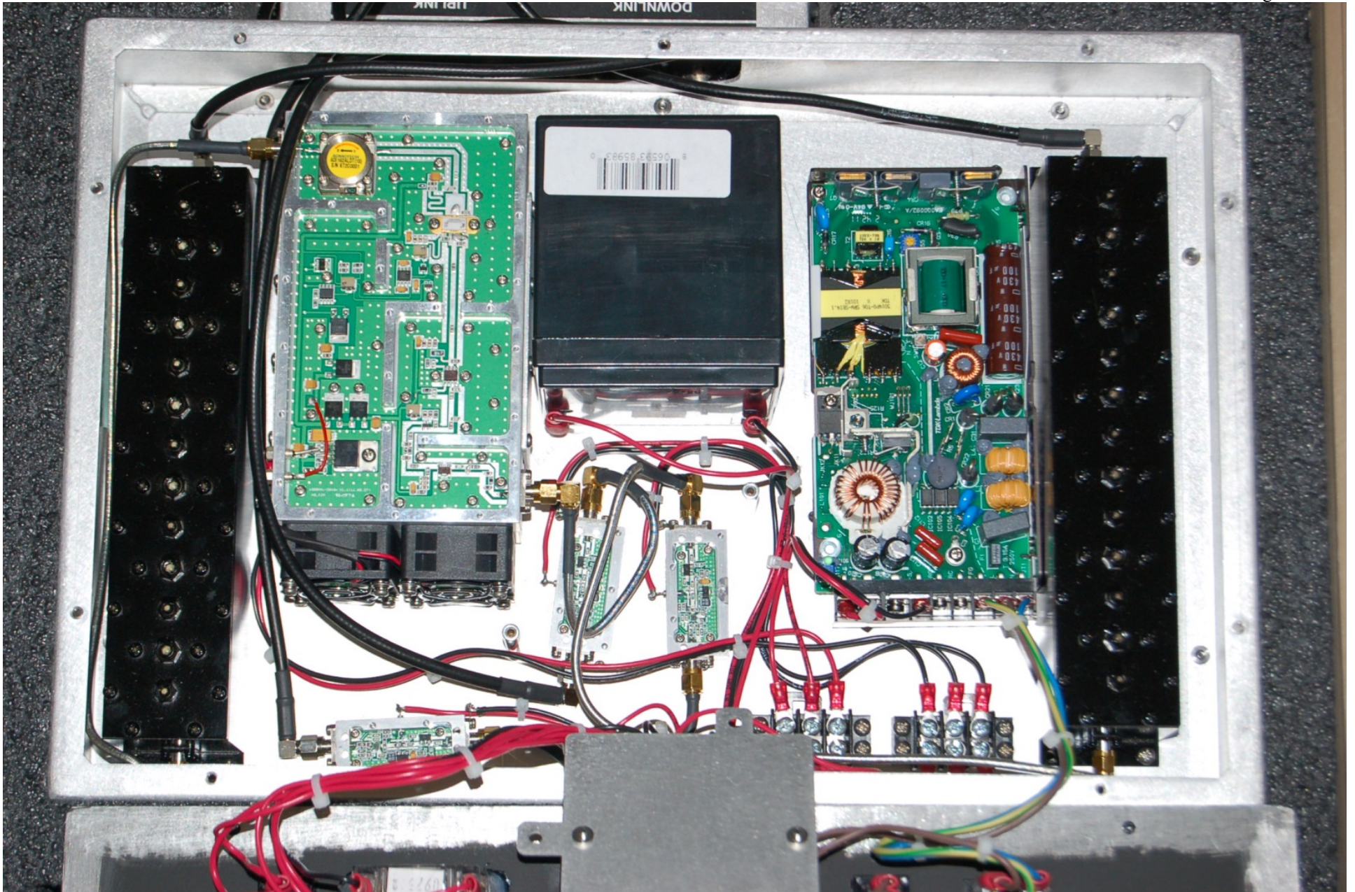
Figure 7 - High Level View with Shields Removed, Note that Black Filters are Sealed
