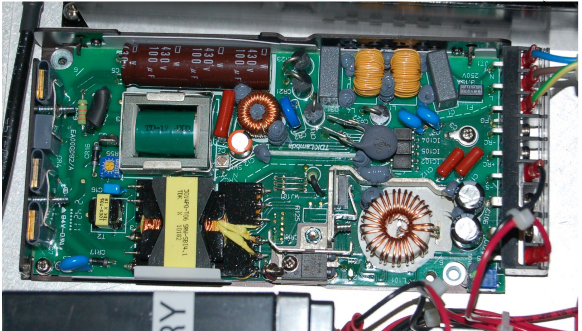
Figure 8 - Power Supply Module - Close Up View
