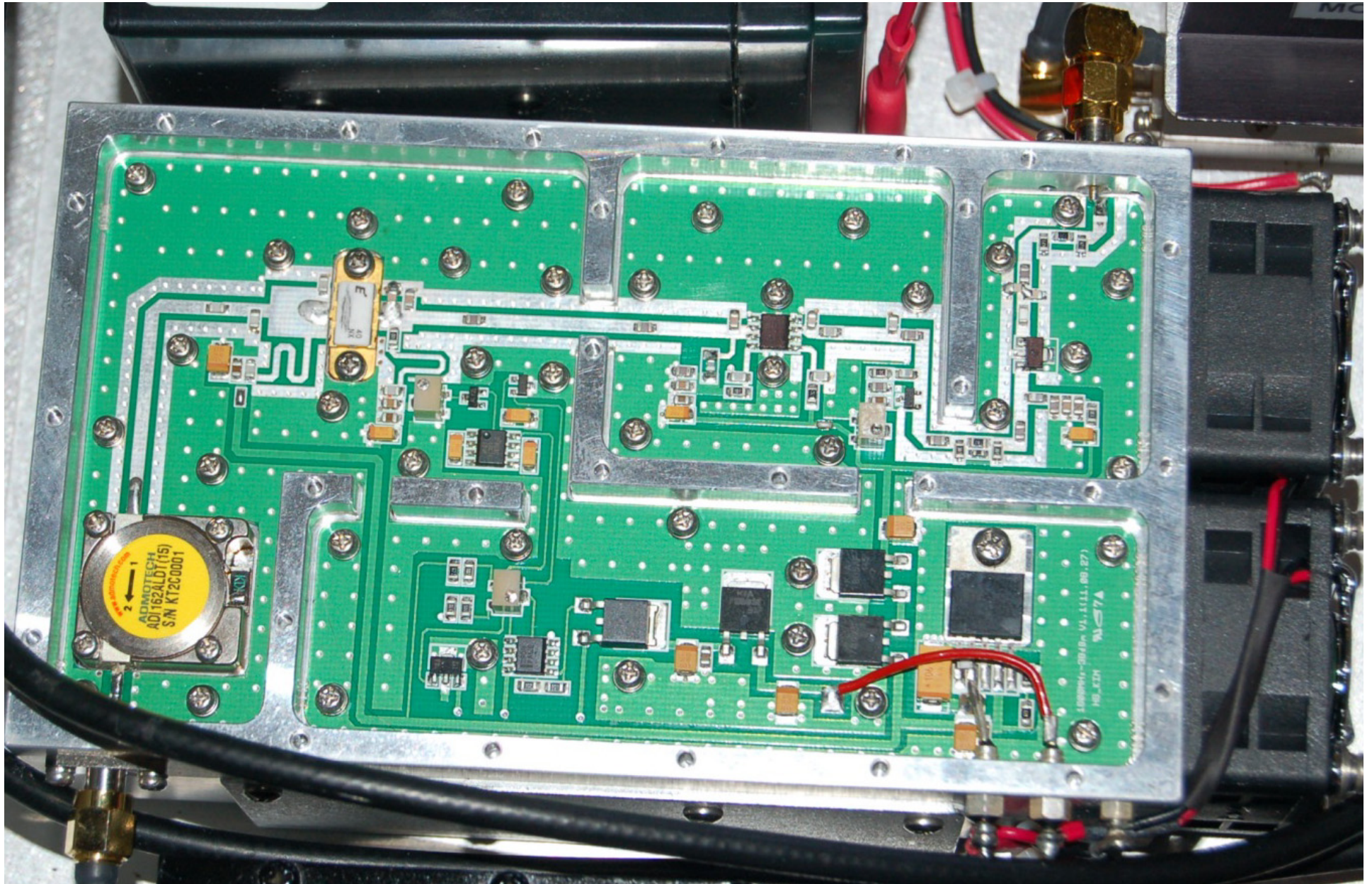
Figure 9 - Power Amp - Close Up View
