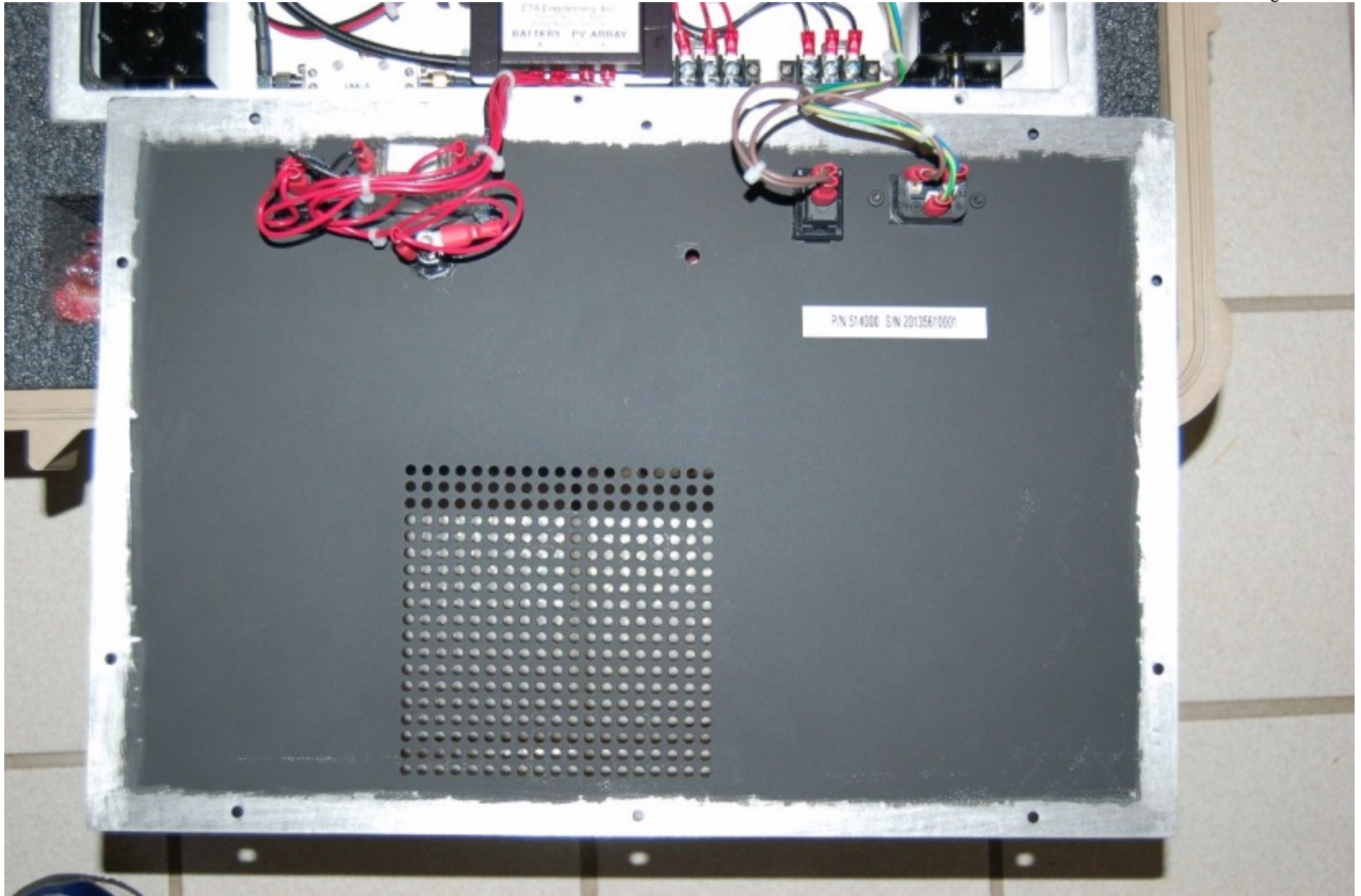
Figure 3 - Front Panel Back Side - Power Switch and Power Entry / Controls
