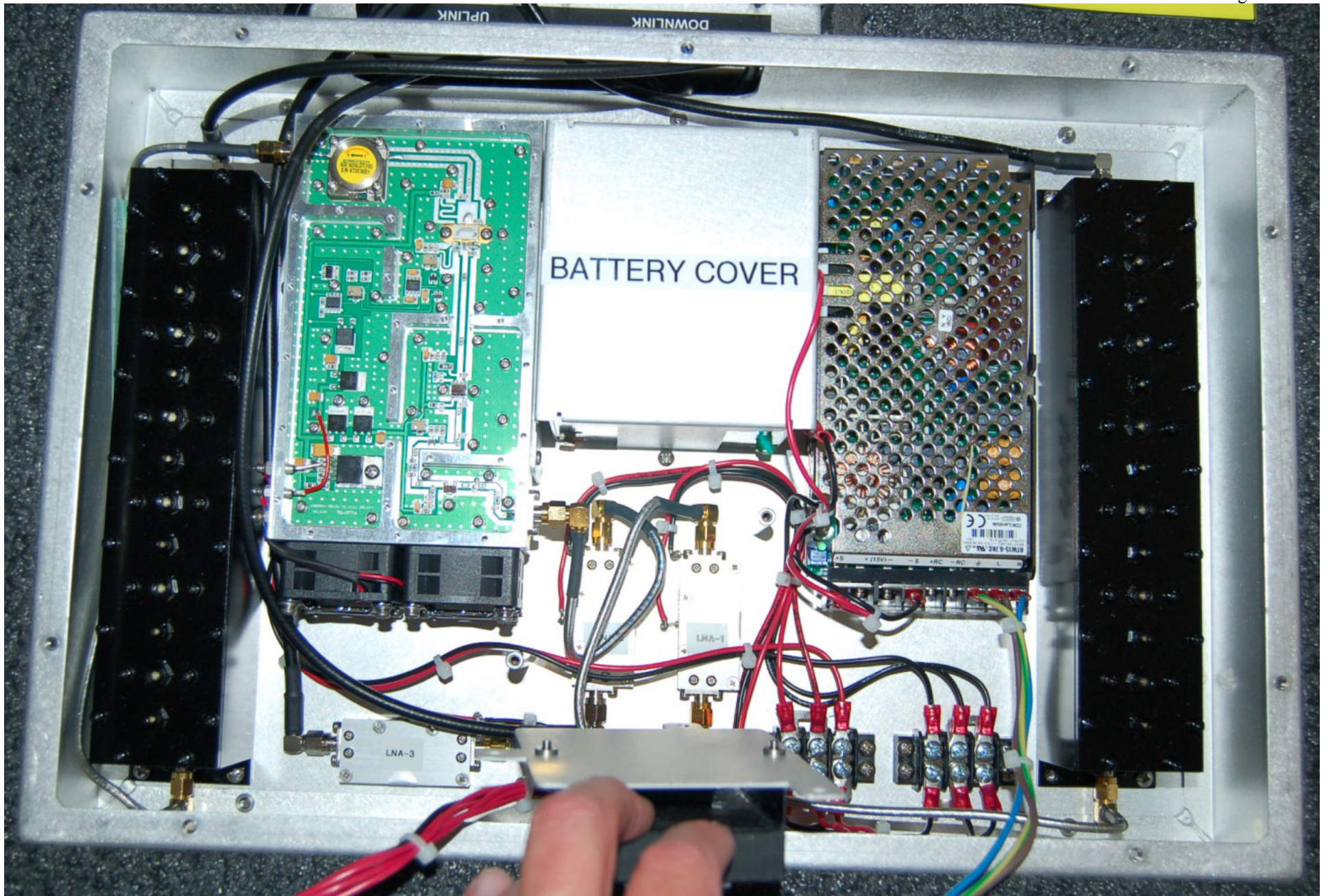
Figure 5 - Power Amp Shield Removed - Charge Controller Lifted to Reveal Low Noise Amps (LNAs)
