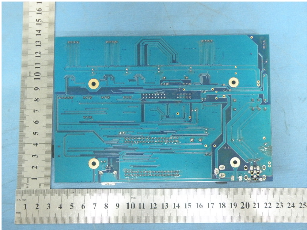
Bottom View
