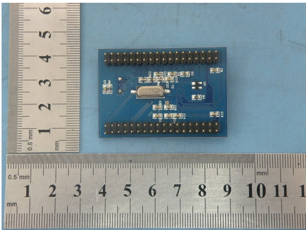
Bottom View
