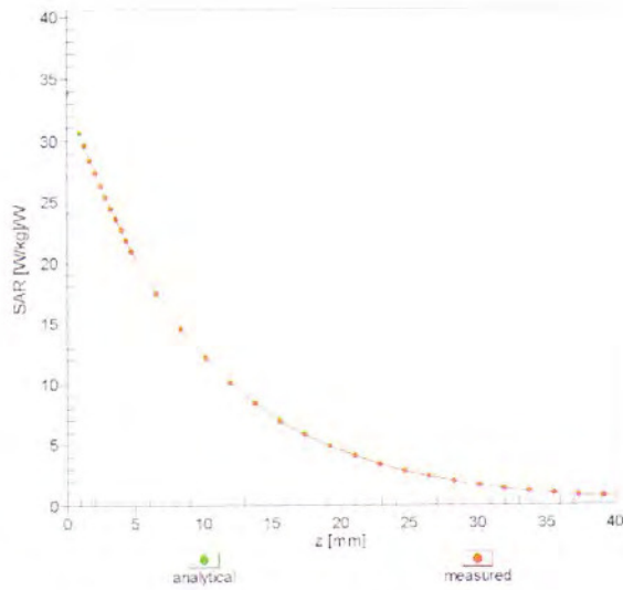
f = 2450 MHz, WGLS R22 (M_convF)
