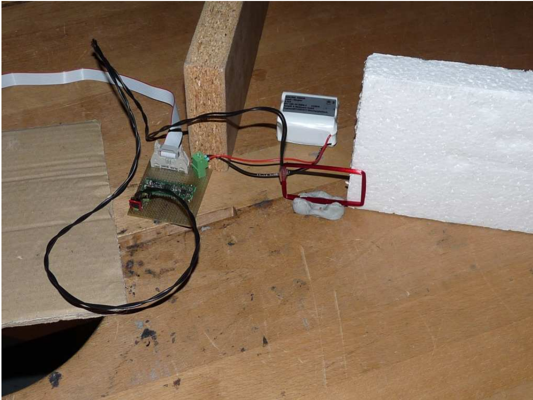
Photo 10: Setup_10, radiated measurements (below 30 MHz) Antenna ANTj01 (04344830)
