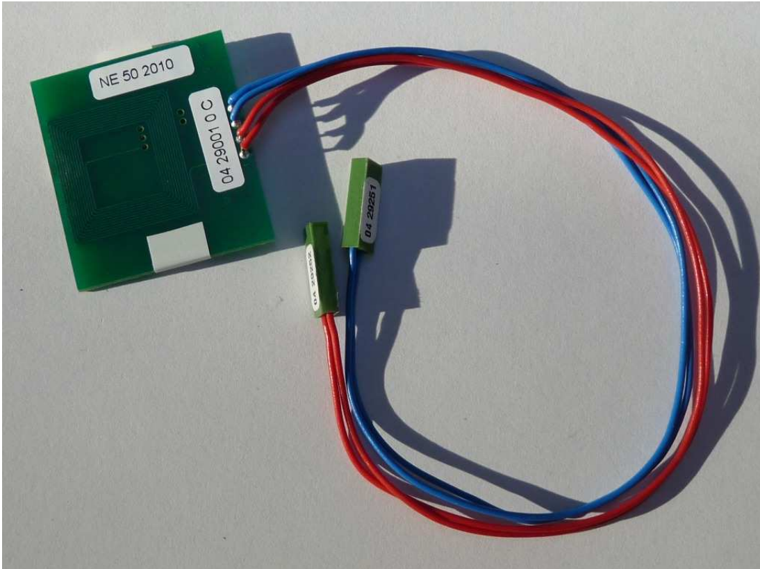
Photo 15: Antenna ANTb01 (04290010)
