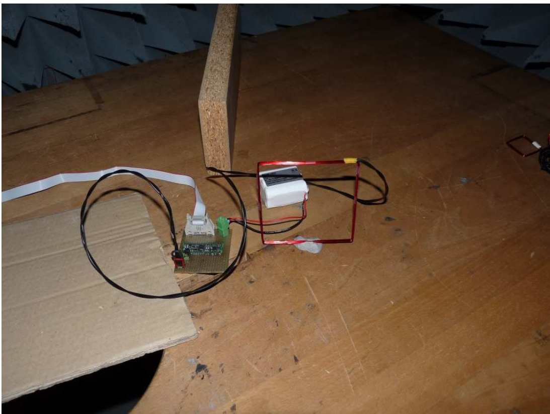
Photo 7: Setup_07, radiated measurements (below 30 MHz) Antenna ANTg01 (04203110)
