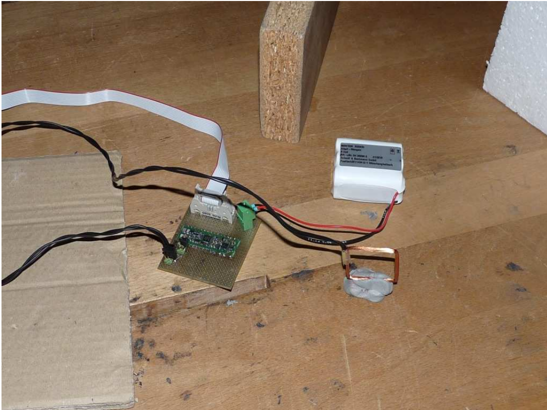
Photo 8: Setup_08, radiated measurements (below 30 MHz) Antenna ANTh01 (04208300)
