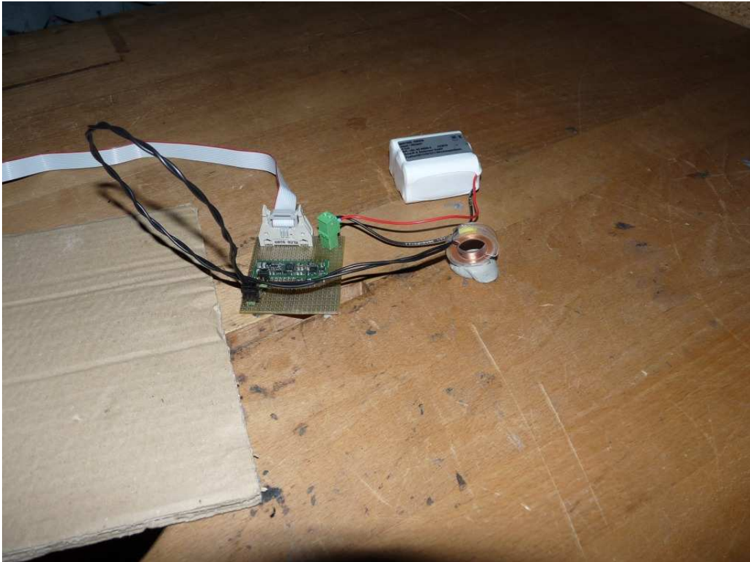
Photo 6: Setup_06, radiated measurements (below 30 MHz) Antenna ANTf01 (04200430)
