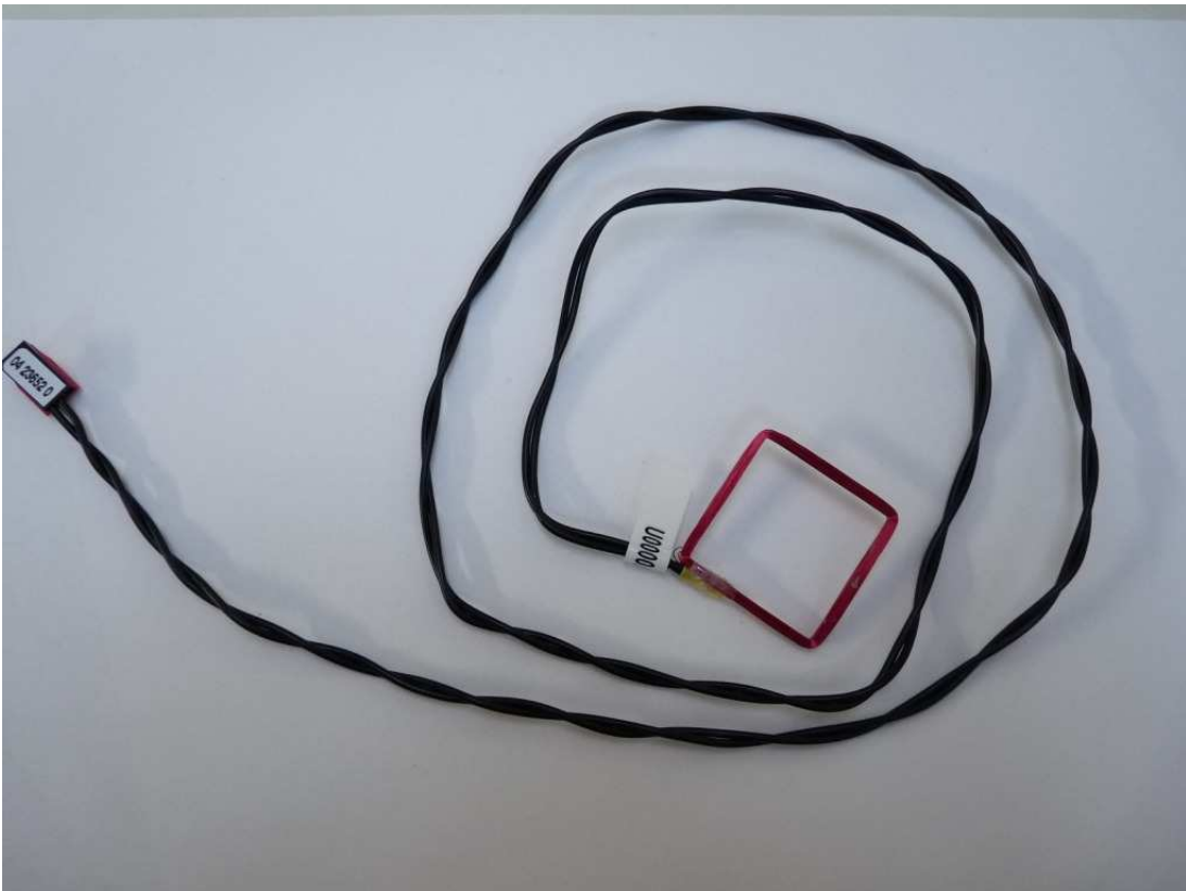
Photo 22: Antenna ANTi01 (04317010)
