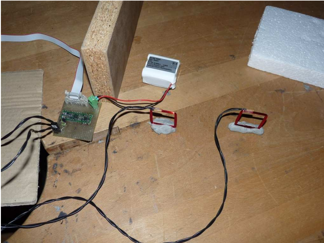
Photo 12: Setup_12, radiated measurements (below 30 MHz) Antenna ANTI01 (04236520)
