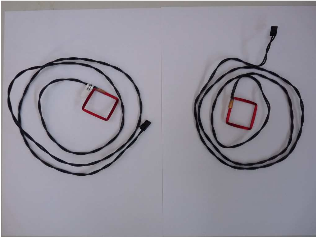
Photo 25: Antenna ANTI01 (04236520)
