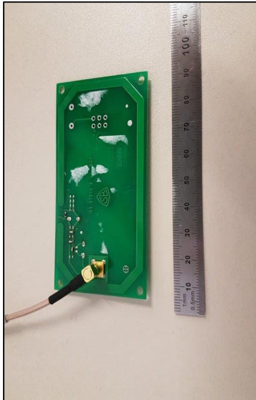
Photo 5: EUT - Antenna 2 - Backside view
