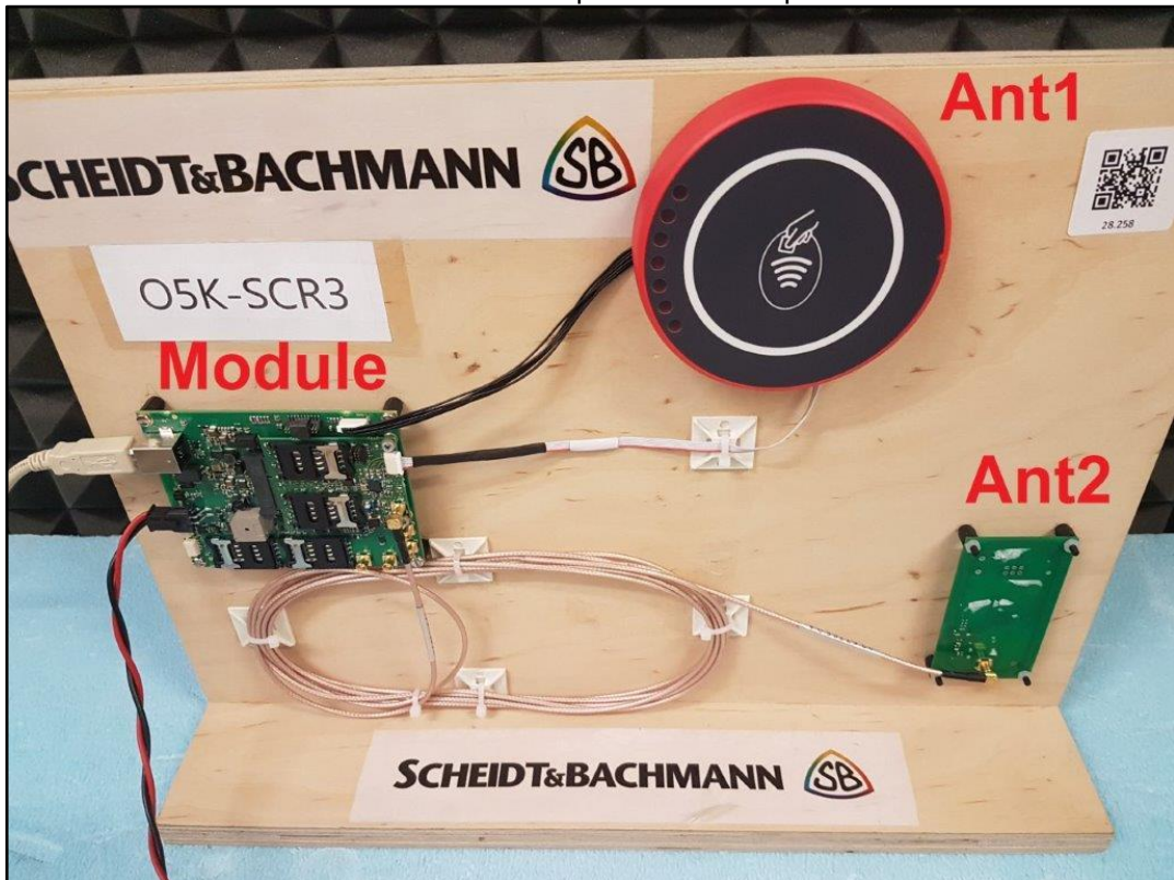
Photo 3: EUT - description of the components
