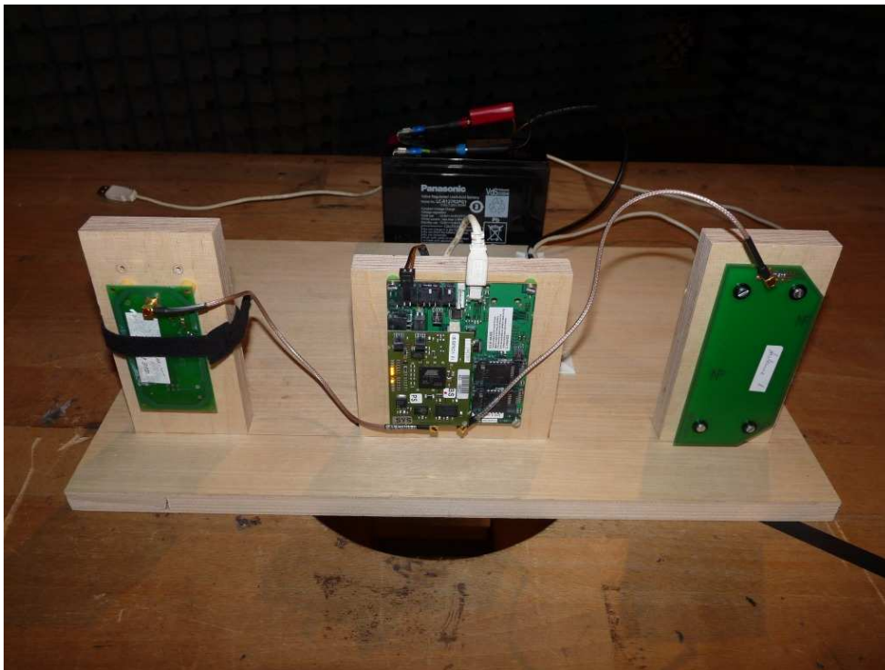
Photo 3: Test setup (Setup 01) for radiated measurements (30 - 140 MHz) with Antenna Basic (0344072) and Antenna Validator (0364127)
