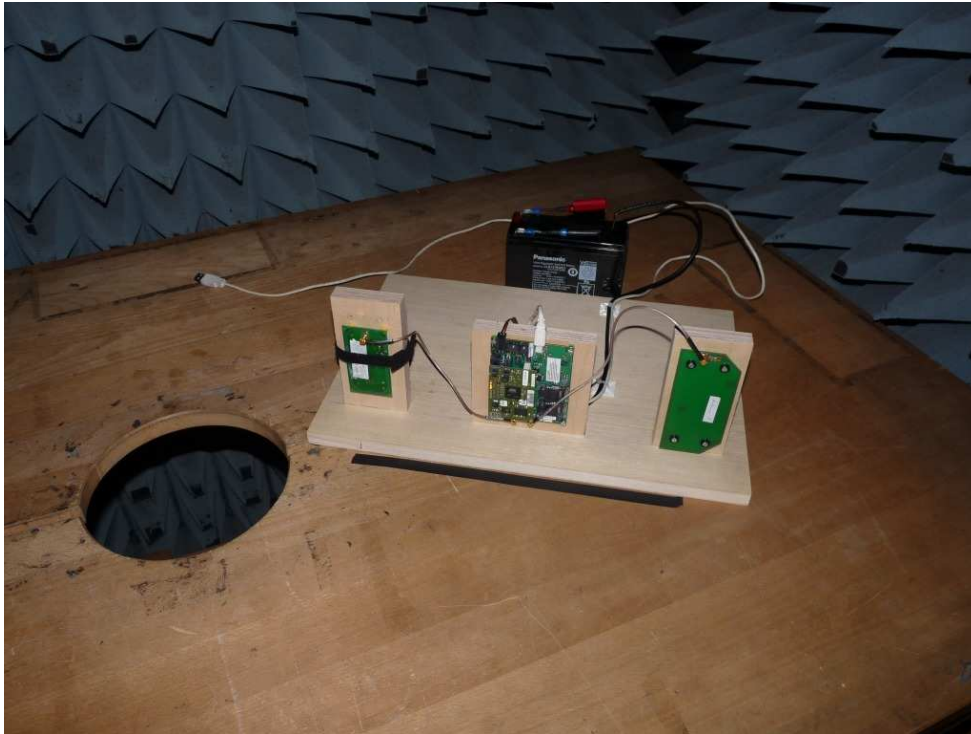
Photo 1: Test setup (Setup 01) for radiated measurements (below 30 MHz) with Antenna Basic (0344072) and Antenna Validator (0364127)
