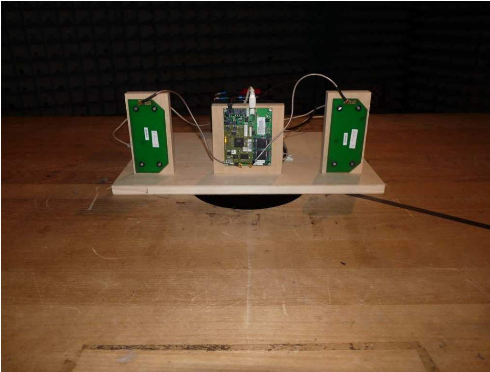
Photo 4: Test setup (Setup 02) for radiated measurements (30 - 140 MHz) with two antennas of Antenna Validator (0364127)
