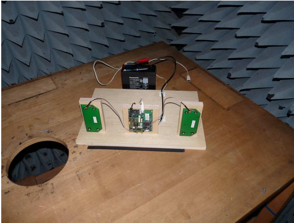
Photo 2: Test setup (Setup 02) for radiated measurements (below 30 MHz) with two antennas of Antenna Validator (0364127)
