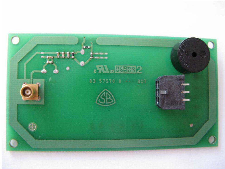
Picture 1. EUT, Antenna
