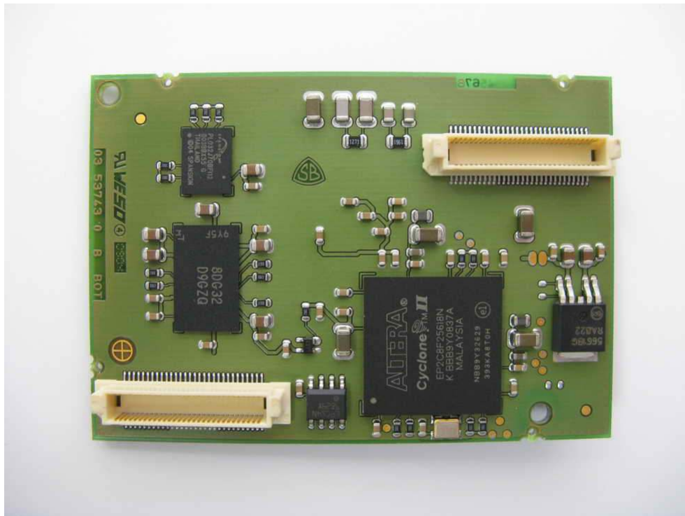
Picture 5. EUT, CPU Modul
