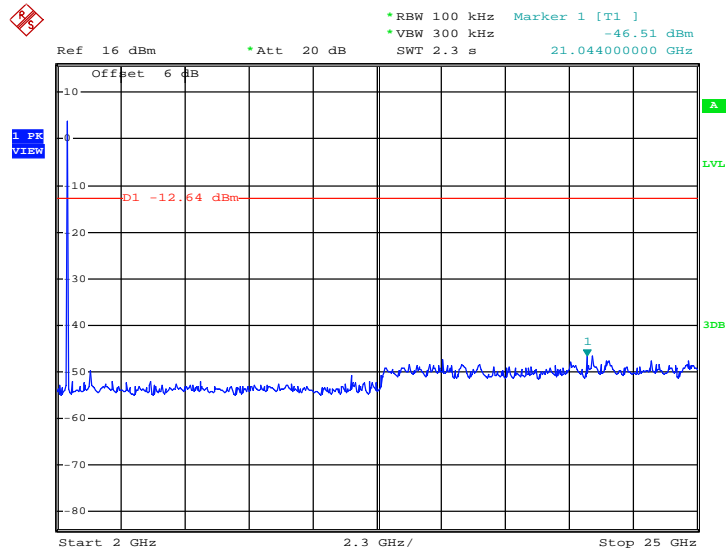
Conducted Spurious Emission Plot on Bluetooth v4.0 LE 1Mbps GFSK Channel 00
