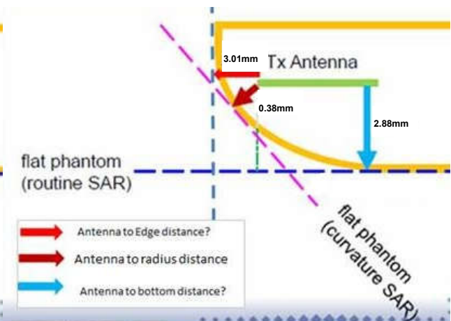
X=3.01mm, Y=2.88mm, Z=0.38mm Exterior Radius Dimension for WLAN
