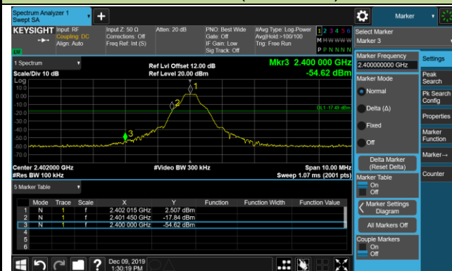
Channel 00 (2402MHz)
