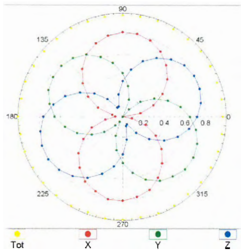
f=600 MHz,TEM
