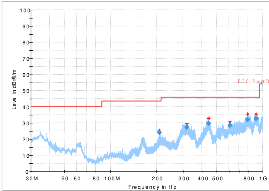
Fig 74. Radiated Spurious Emission (802.11 n-40MHz,Ch1,30MHz~1GHz)
