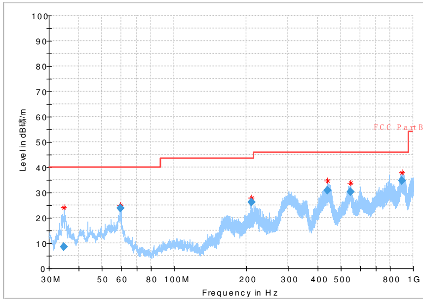
Fig 64. Radiated Spurious Emission (802.11g,Ch1,30MHz~1GHz)
