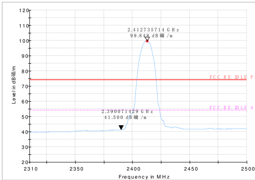
Fig 62. Radiated emission (Power): 802.11g, low channel
