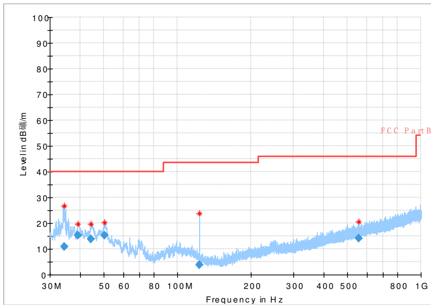
Fig 59. Radiated Spurious Emission (802.11b,Ch1,30MHz~1GHz)
