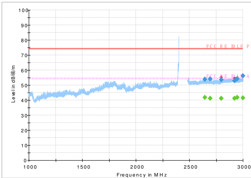
Fig 75. Radiated Spurious Emission (802.11 n-40MHz,Ch1,1GHz~3GHz)
