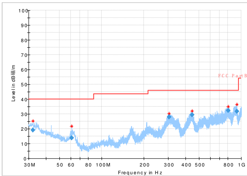
Fig 69. Radiated Spurious Emission (802.11 n-20MHz,Ch1,30MHz~1GHz)
