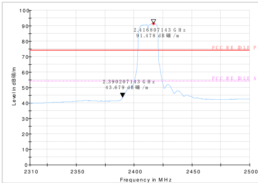
Fig 72. Radiated emission (Power): 802.11n (40M) , low channel
