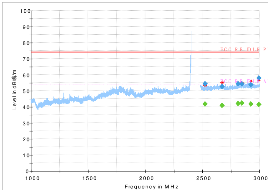
Fig 65. Radiated Spurious Emission (802.11g,Ch1,1GHz~3GHz)
