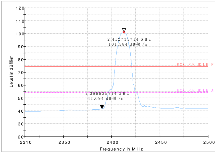
Fig 57. Radiated emission (Power): 802.11b, low channel
