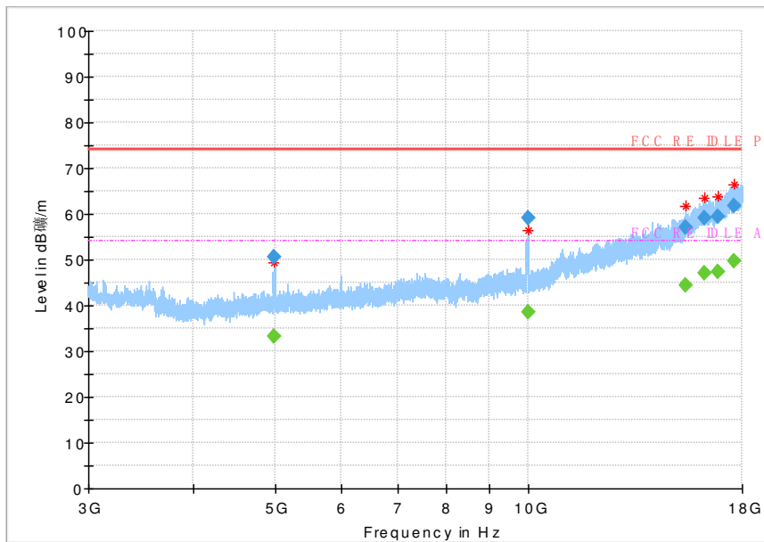
Fig 76. Radiated Spurious Emission (802.11 n-40MHz,Ch1,3GHz~18GHz)
