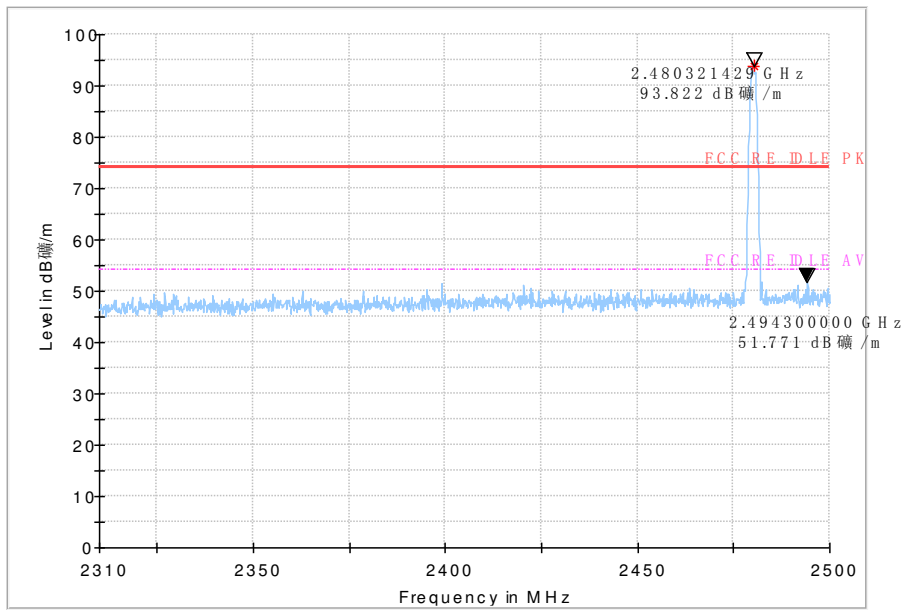
Peak detector Bandedge:ch39
