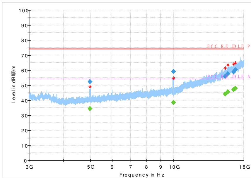
Fig.23 Radiated emission: Ch39, 3GHz~18GHz
