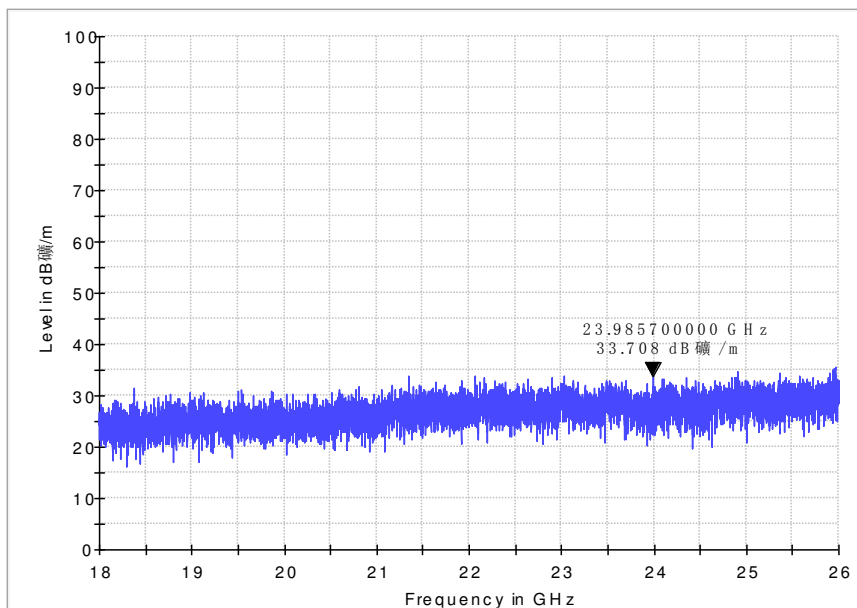
Fig.24 Radiated emission: Ch0, 18GHz~26GHz
