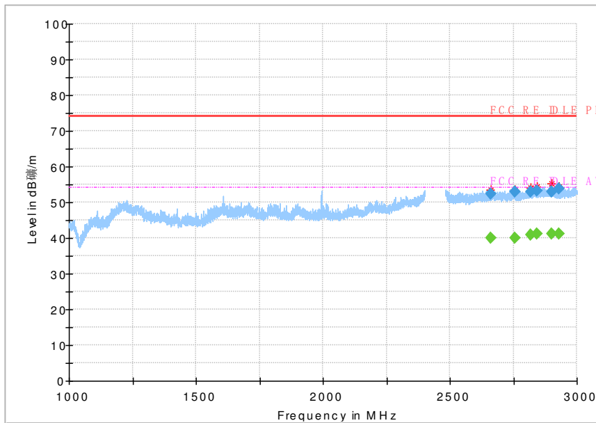
Fig.22 Radiated emission: Ch39, 1GHz~3GHz
