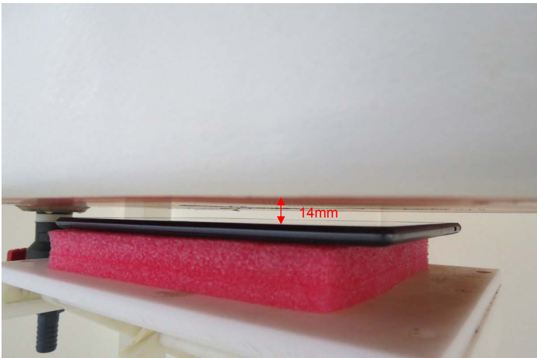
Picture 13: Front Side, the distance from handset to the bottom of the Phantom is 14mm
