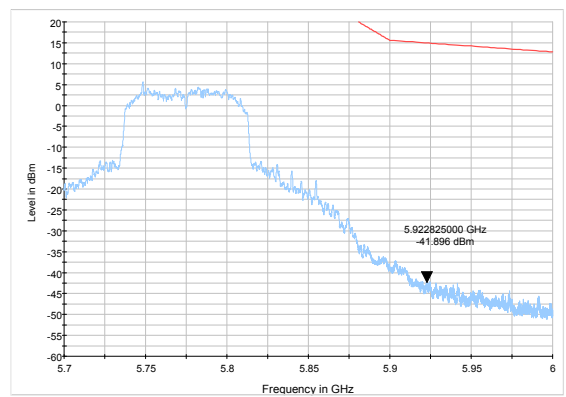
802.11ac HT80- Channel 155: Peak
