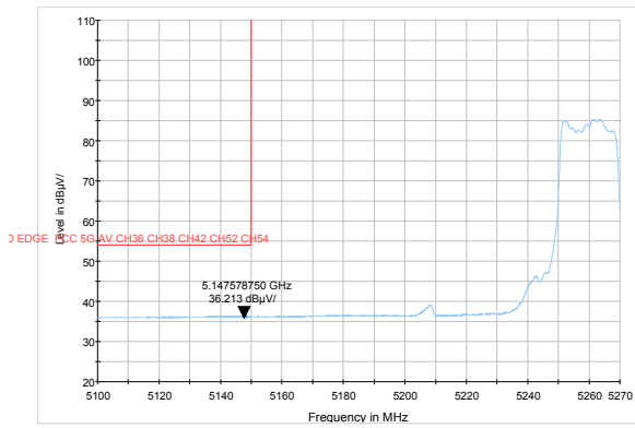
802.11n HT40-Channel 54: Peak
