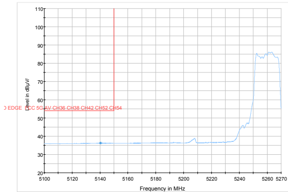
802.11n HT20-Channel 52: Peak
