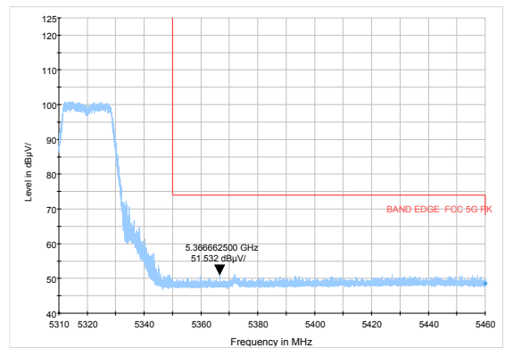
802.11n HT20-Channel 64: Peak
