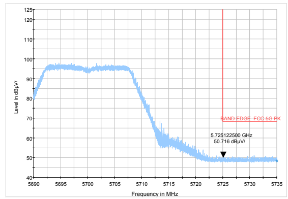
802.11a-Channel 140: Peak
