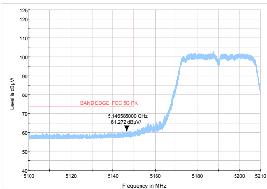
802.11ac HT40-Channel 38: Peak
