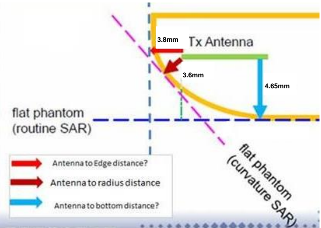
Curved Surface of Edge1, Test Separation 0 mm
