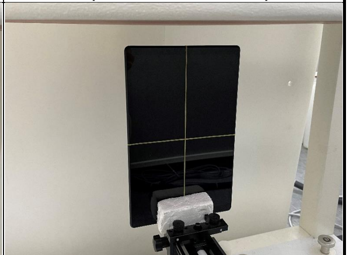
Top Side of EUT with 2.5 cm Gap
