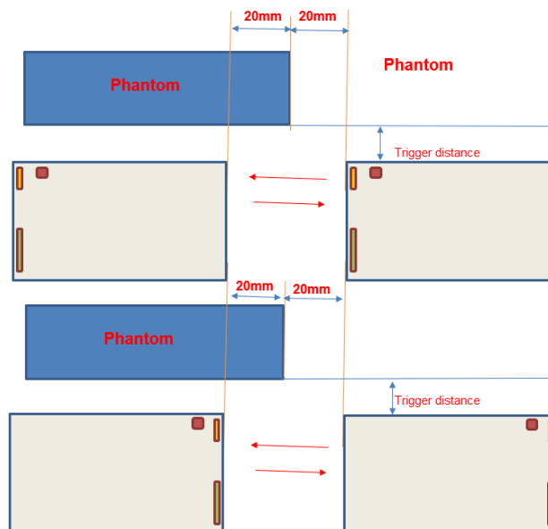
proximity sensor coverage assesment (Y coordinate direction)
