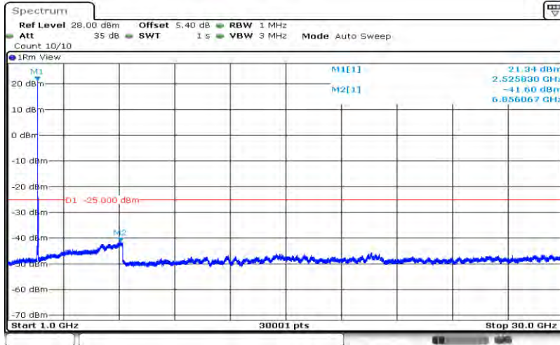
Band7-20MHz-64QAM-21100-1RB#0-Range2:1000~30000MHz
