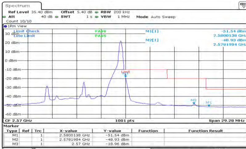
Band7-10MHz-QPSK-21400-50RB#0
