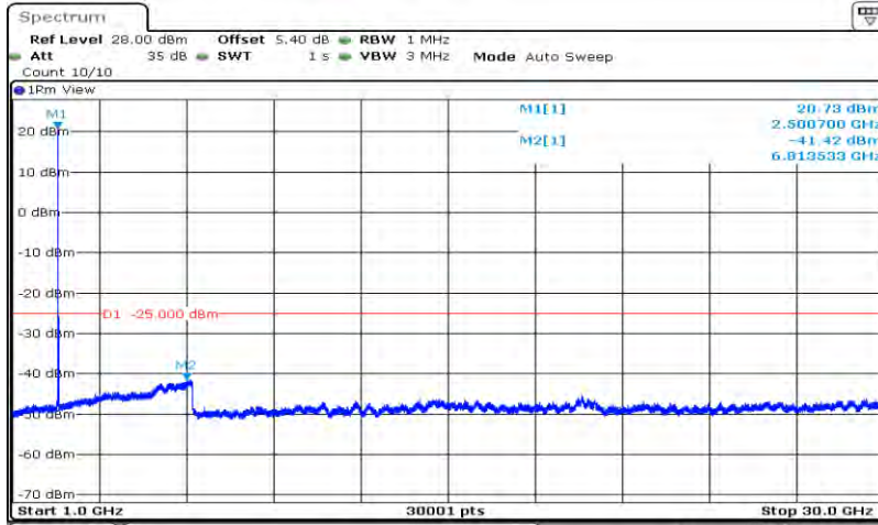
Band7-20MHz-16QAM-20850-1RB#0-Range2:1000~30000MHz
