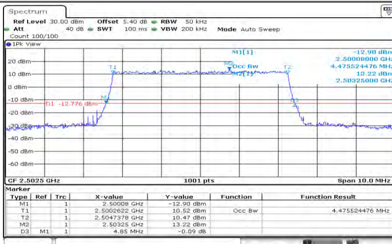
Band7-5MHz-QPSK-20775-25RB#0-4.476
