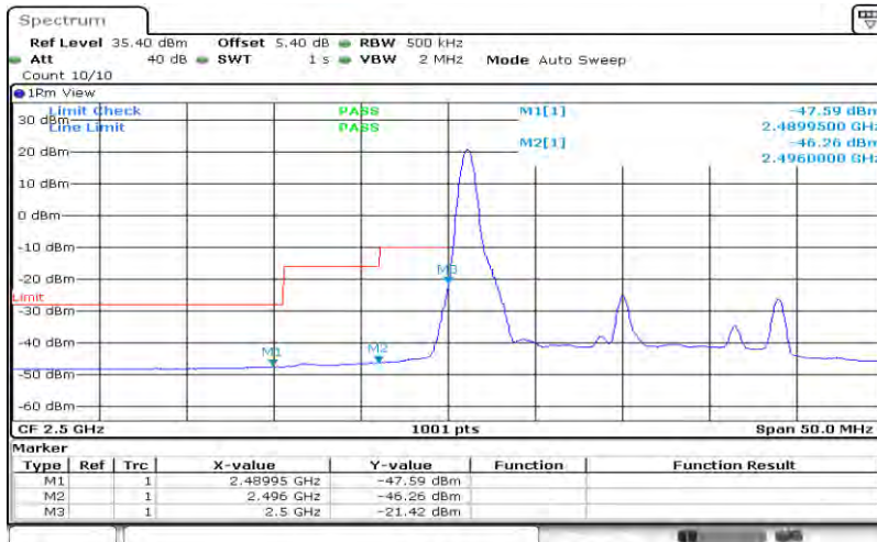
Band7-20MHz-64QAM-20850-100RB#0
