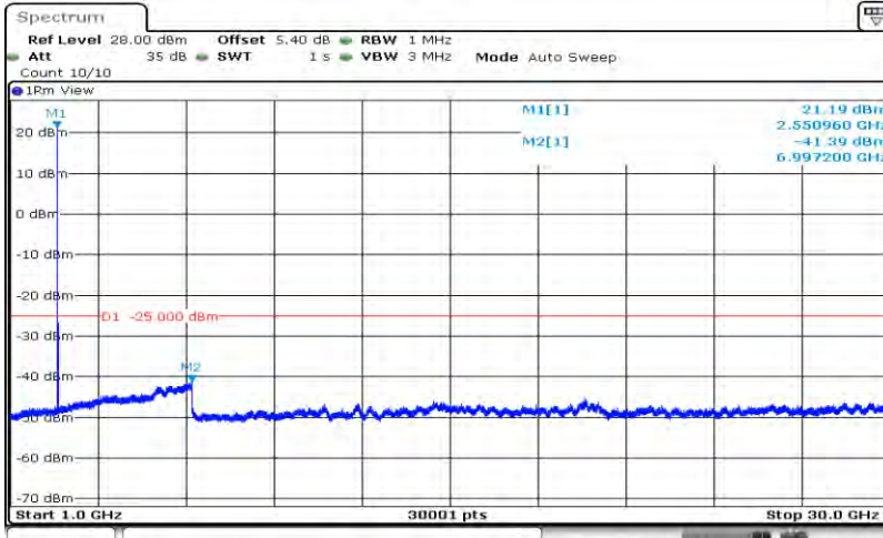
Band7-20MHz-64QAM-21350-1RB#0-Range2:1000~30000MHz
