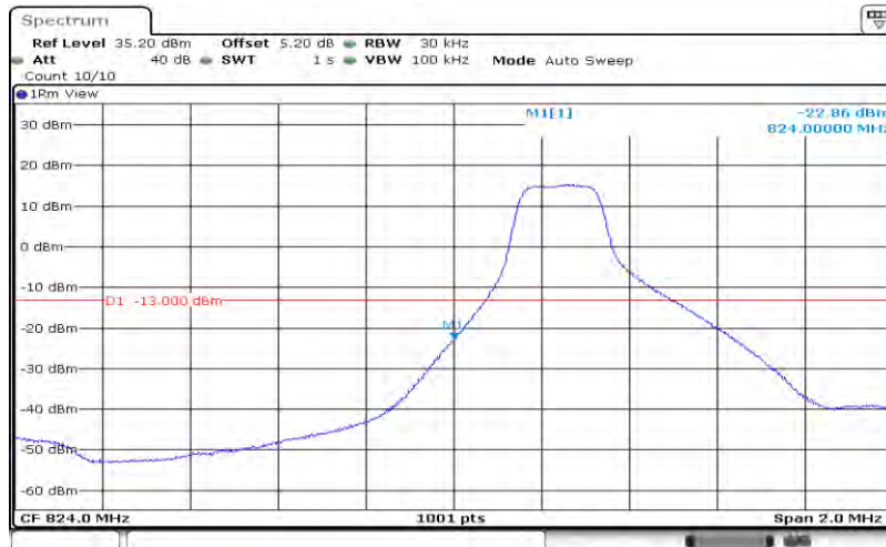
Band5-3MHz-16QAM-20415-15RB#0
