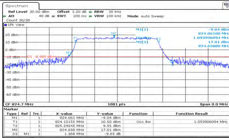
Band5-1.4MHz-QPSK-20407-6RB#0-1.094
