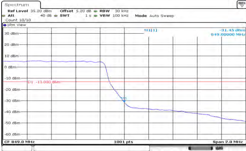
Band5-1.4MHz-64QAM-20643-6RB#0
