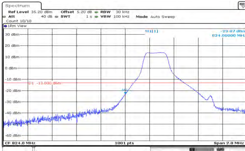
Band5-1.4MHz-64QAM-20407-6RB#0
