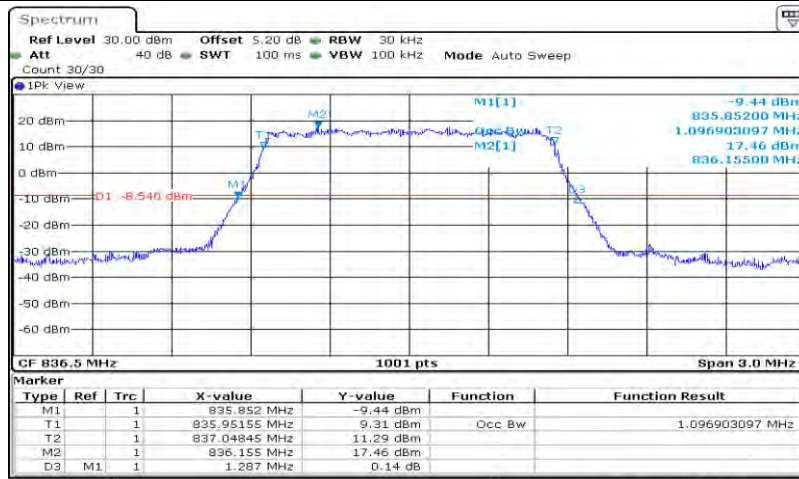
Band5-1.4MHz-QPSK-20525-6RB#0-1.097
