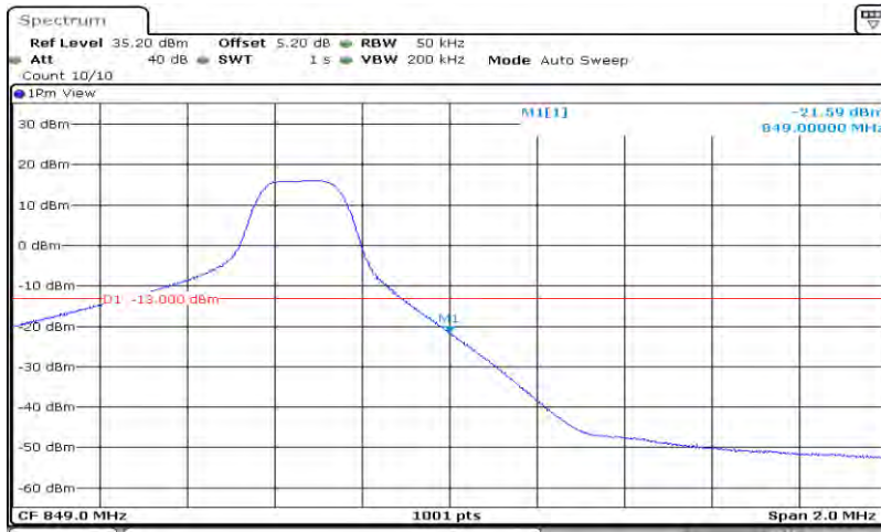
Band5-5MHz-64QAM-20625-25RB#0
