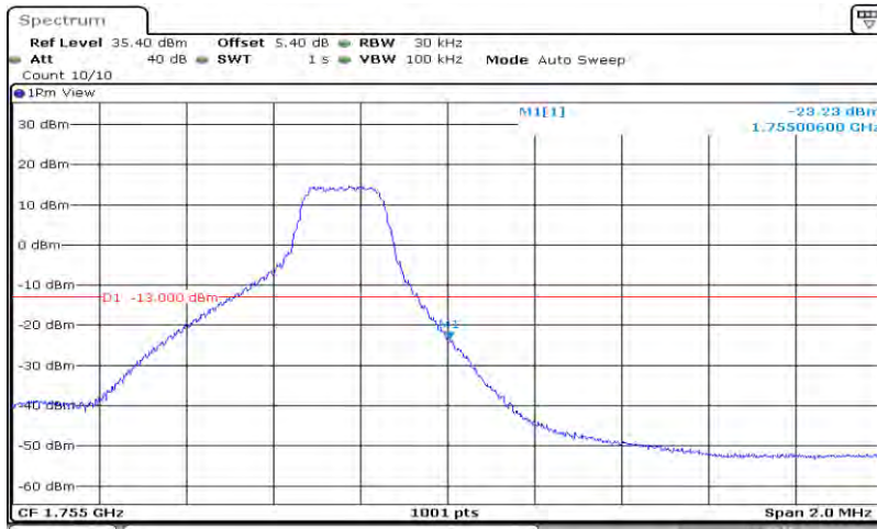
Band4-3MHz-64QAM-20385-15RB#0
