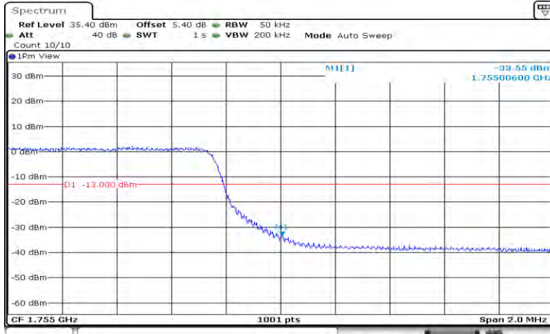
Band4-5MHz-64QAM-20375-25RB#0
