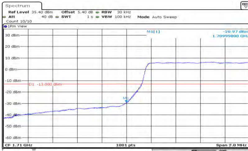
Band4-1.4MHz-64QAM-19957-6RB#0
