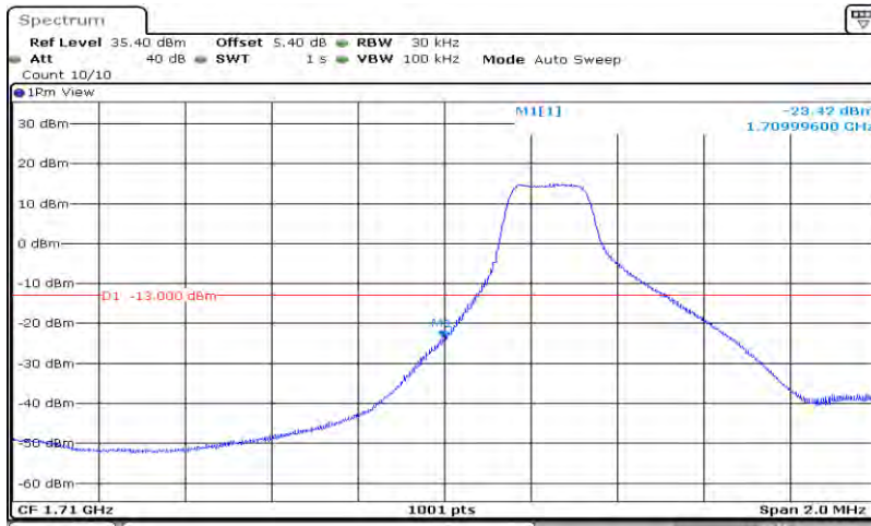
Band4-3MHz-64QAM-19965-15RB#0
