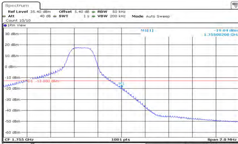
Band4-5MHz-16QAM-20375-25RB#0
