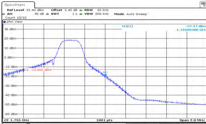
Band4-5MHz-QPSK-20375-25RB#0
