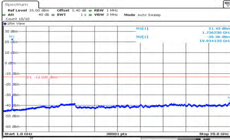
Band4-20MHz-64QAM-20300-1RB#0-Range2:1000~20000MHz
