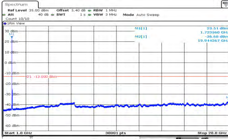
Band4-20MHz-64QAM-20175-1RB#0-Range2:1000~20000MHz
