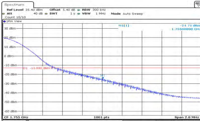
Band4-20MHz-64QAM-20300-100RB#0
