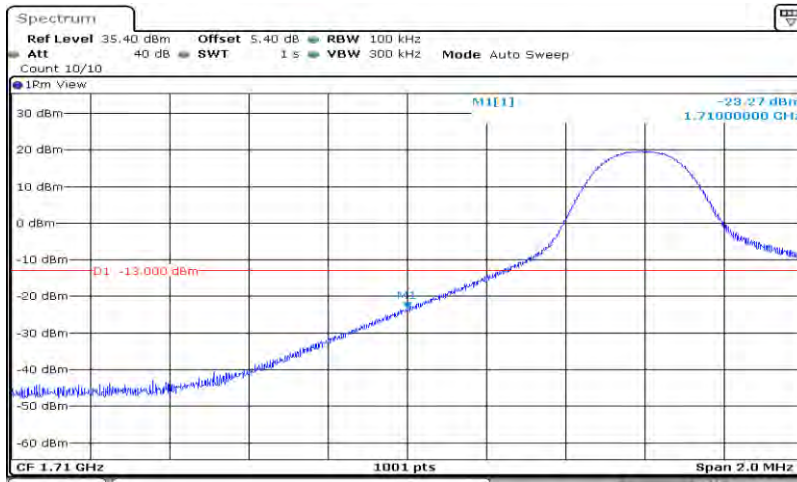
Band4-10MHz-64QAM-20000-50RB#0
