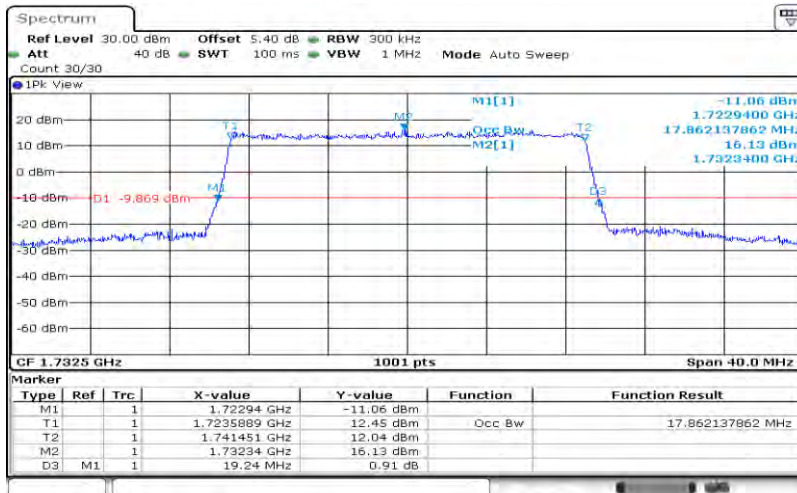
Band4-20MHz-QPSK-20175-100RB#0-17.862
