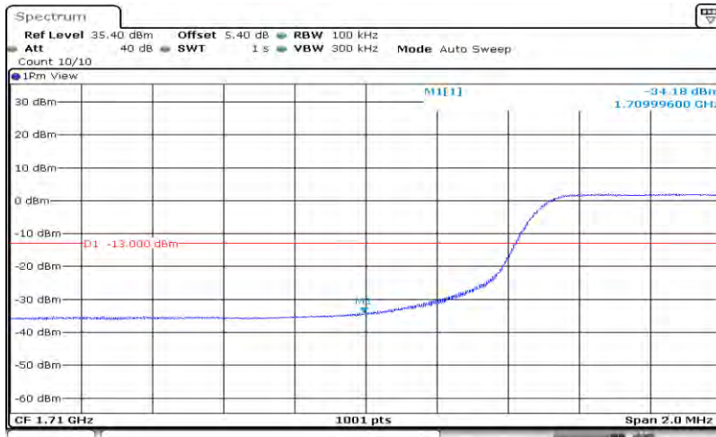
Band4-10MHz-64QAM-20000-50RB#0
