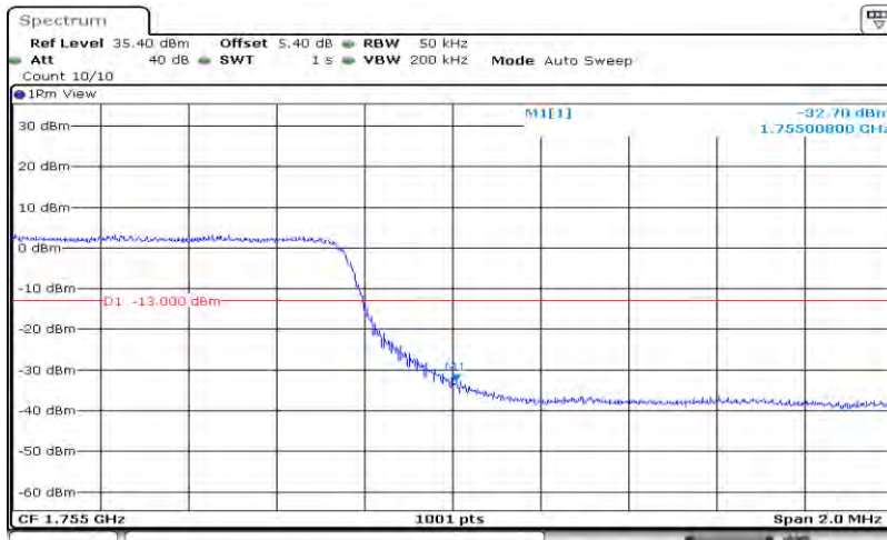
Band4-5MHz-16QAM-20375-25RB#0
