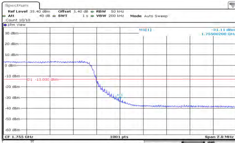
Band4-5MHz-QPSK-20375-25RB#0
