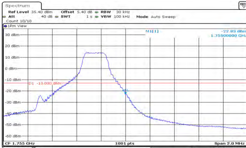
Band4-1.4MHz-64QAM-20393-6RB#0
