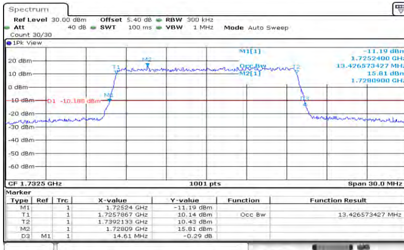
Band4-15MHz-64QAM-20175-75RB#0-13.427
