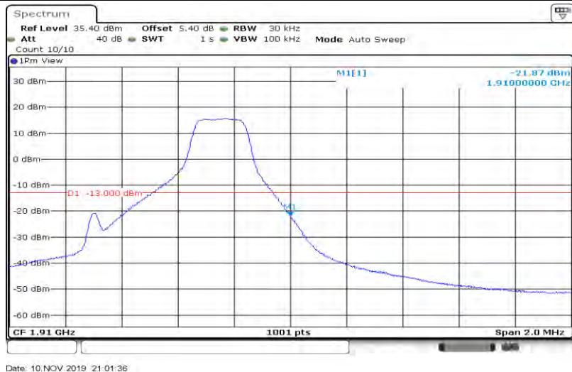
Band2-1.4MHz-16QAM-19193-6RB#0
