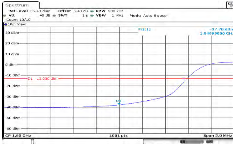
Band2-15MHz-64QAM-18675-75RB#0
