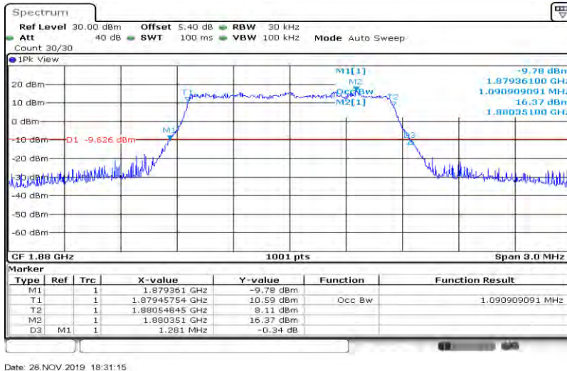
Band2-1.4MHz-64QAM-19193-6RB#0-1.091
