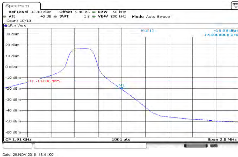
Band2-5MHz-64QAM-19175-25RB#0
