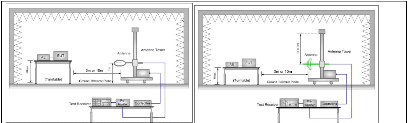
Figure 1. Below 30MHz
