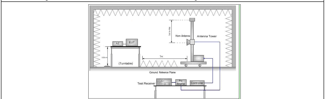
Figure 3. Above 1 GHz
