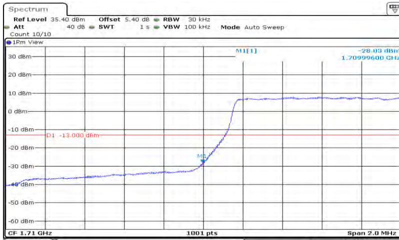
Band4-1.4MHz-16QAM-19957-6RB#0
