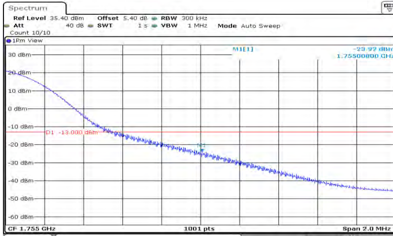
Band4-20MHz-64QAM-20300-100RB#0
