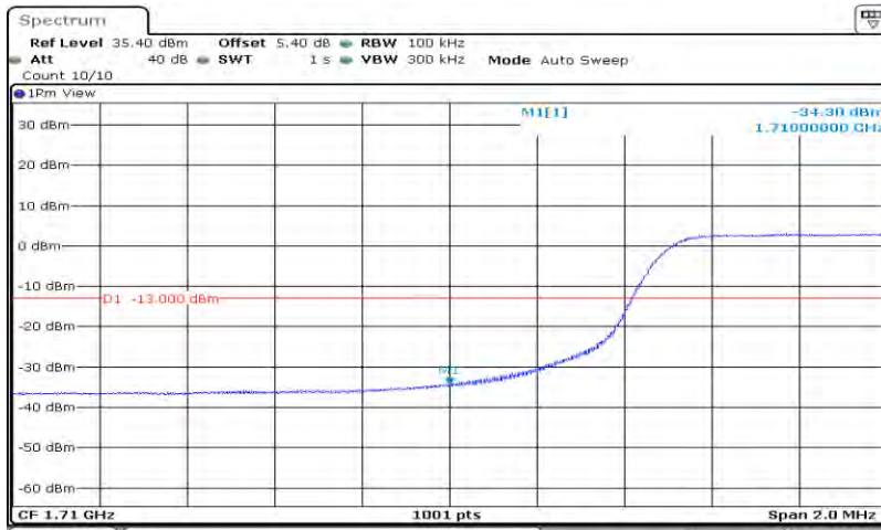
Band4-10MHz-16QAM-20000-50RB#0
