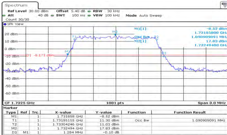
Band4-1.4MHz-QPSK-20175-6RB#0-1.091
