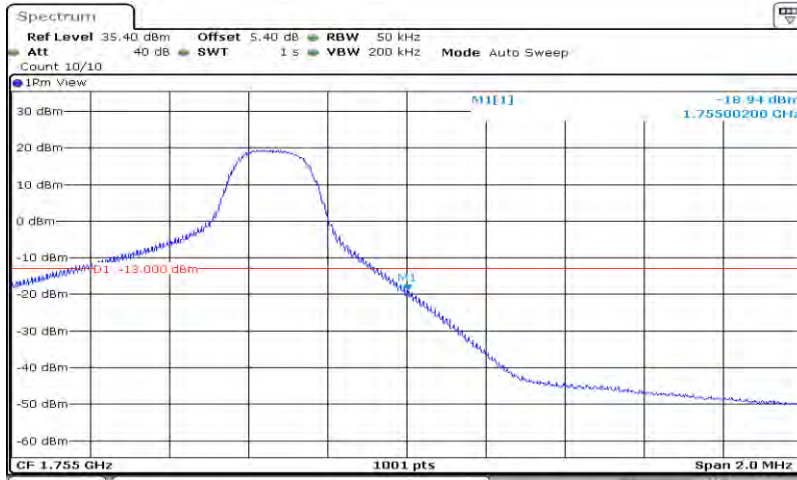
Band4-5MHz-QPSK-20375-25RB#0
