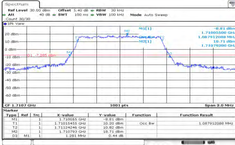
Band4-1.4MHz-QPSK-19957-6RB#0-1.088
