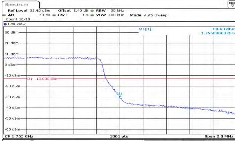
Band4-1.4MHz-64QAM-20393-6RB#
