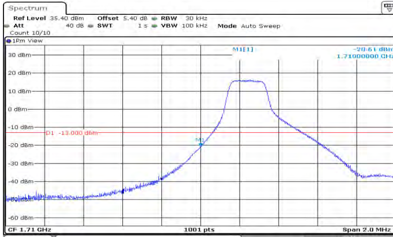
Band4-3MHz-16QAM-19965-15RB#0
