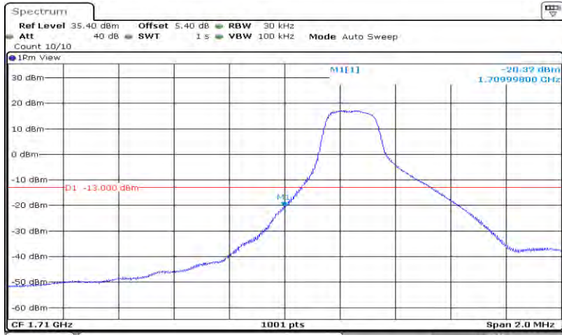
Band4-3MHz-QPSK-19965-15RB#0
