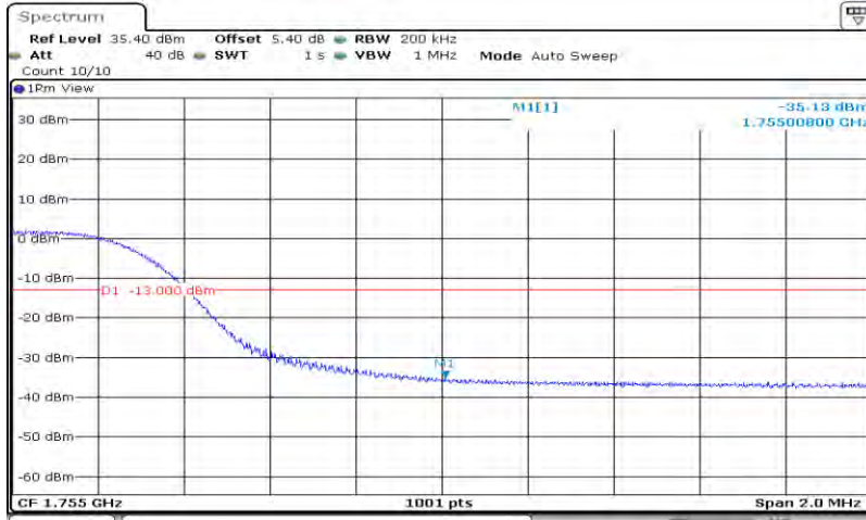
Band4-15MHz-64QAM-20325-75RB#0
