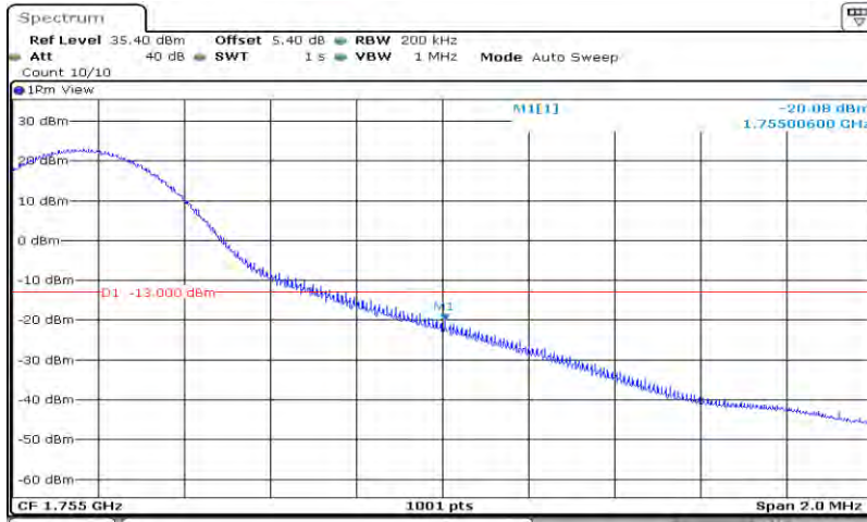
Band4-15MHz-16QAM-20325-75RB#0
