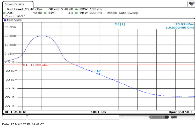
Band2-10MHz-16QAM-19150-50RB#0
