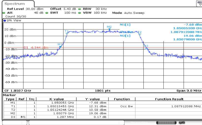
Band2-1.4MHz-QPSK-18607-6RB#0-1.088
