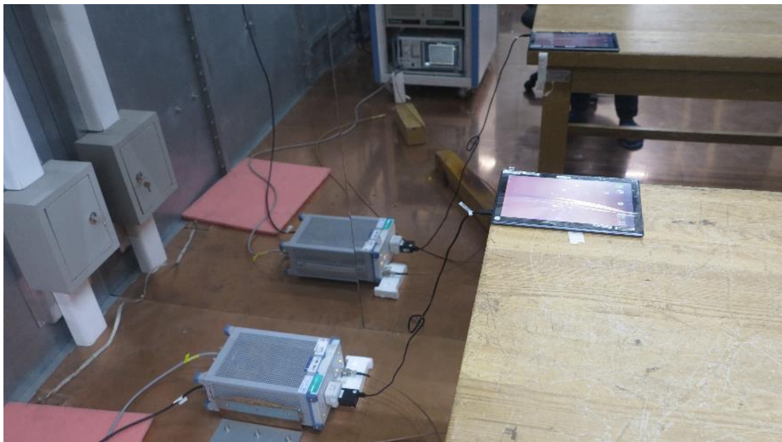
Part15C conducted emission
