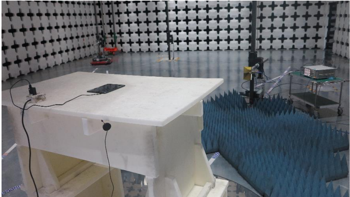
Part15C radiated emission
