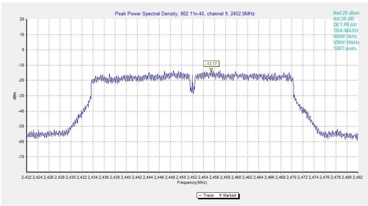
Fig.B.3.12 Power Spectral Density (802.11n-HT40, Ch 9)
