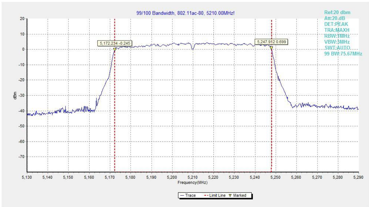
Fig.39 99% Occupied bandwidth (802.11ac-HT80, 5210MHz)
