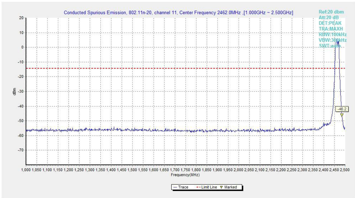
Fig.A.6.1.19 Transmitter Spurious Emission - Conducted (802.11n-HT20, Ch11, 1 GHz-2.5 GHz)
