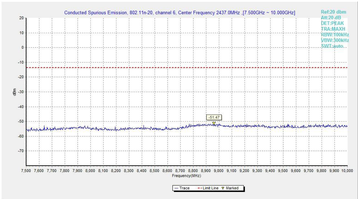
Fig.A.6.1.13 Transmitter Spurious Emission - Conducted (802.11n-HT20, Ch6, 7.5 GHz-10 GHz)
