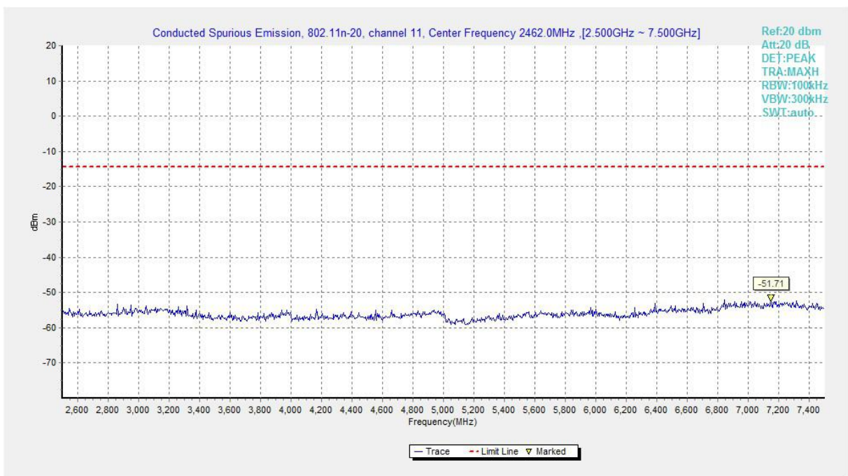
Fig.A.6.1.20 Transmitter Spurious Emission - Conducted (802.11n-HT20, Ch11, 2.5 GHz-7.5 GHz)
