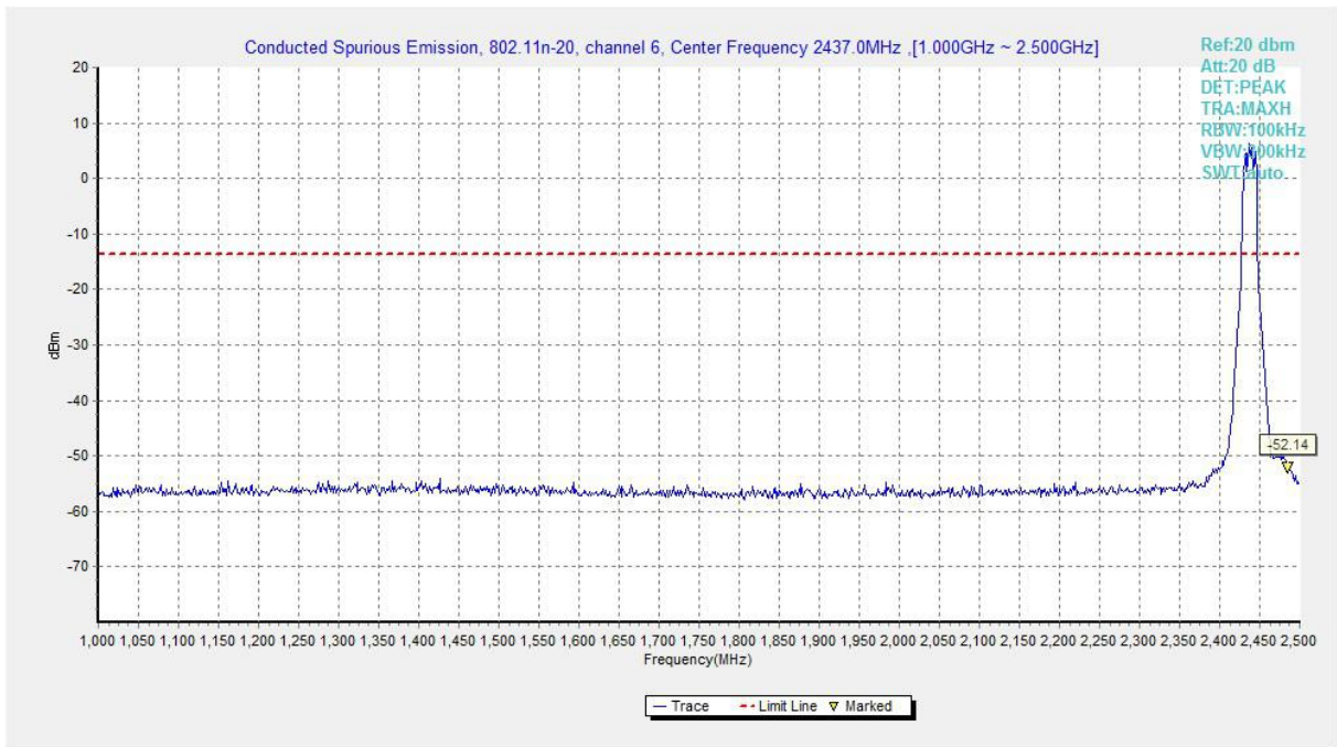
Fig.A.6.1.11 Transmitter Spurious Emission - Conducted (802.11n-HT20, Ch6, 1 GHz-2.5 GHz)
