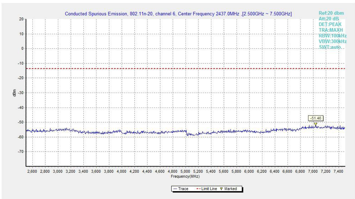
Fig.A.6.1.12 Transmitter Spurious Emission - Conducted (802.11n-HT20, Ch6, 2.5 GHz-7.5 GHz)
