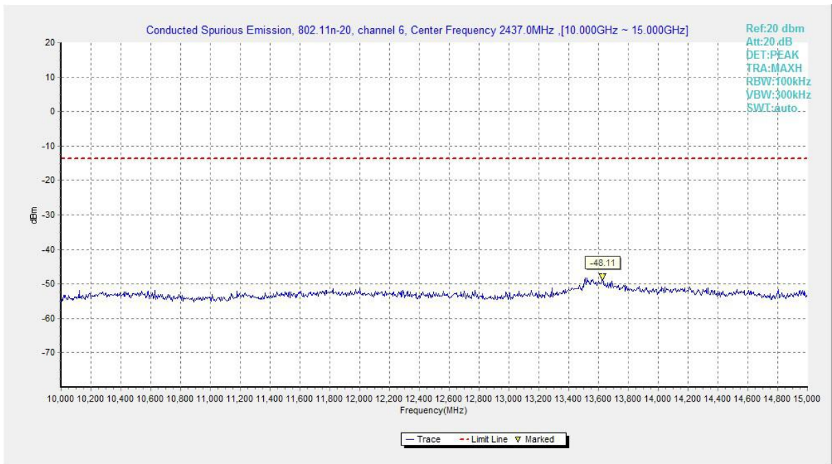
Fig.A.6.1.14 Transmitter Spurious Emission - Conducted (802.11n-HT20, Ch6, 10 GHz-15 GHz)
