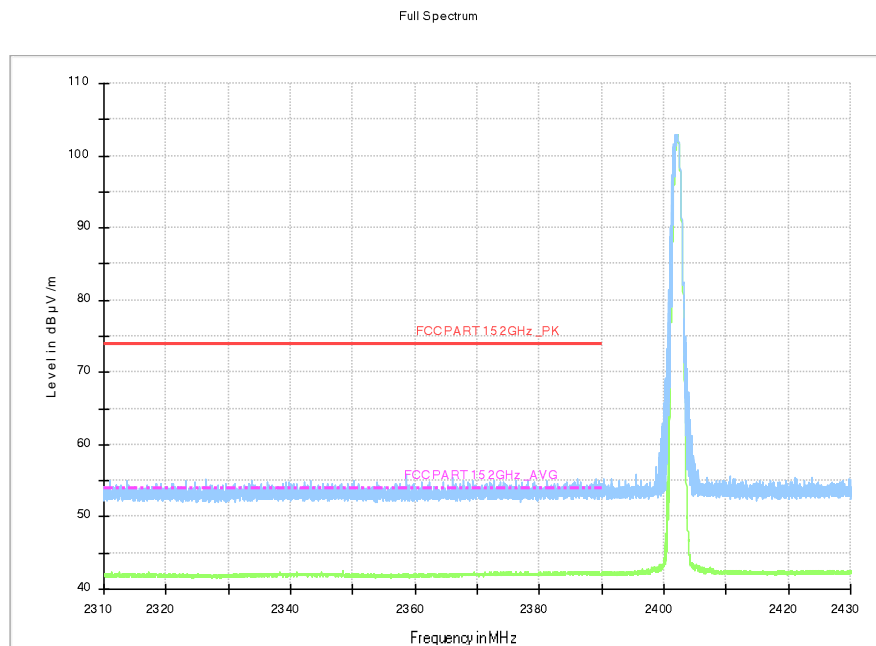
Fig.13. Frequency Band Edges: GFSK, Channel 0, Hopping Off, 2.31 GHz – 2.43GHz
