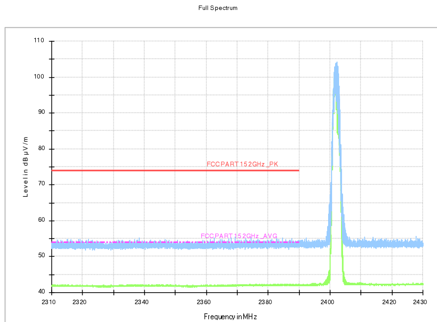
Fig.15. Frequency Band Edges: \pi/4 DQPSK, Channel 0, Hopping Off, 2.31 GHz - 2.43GHz
