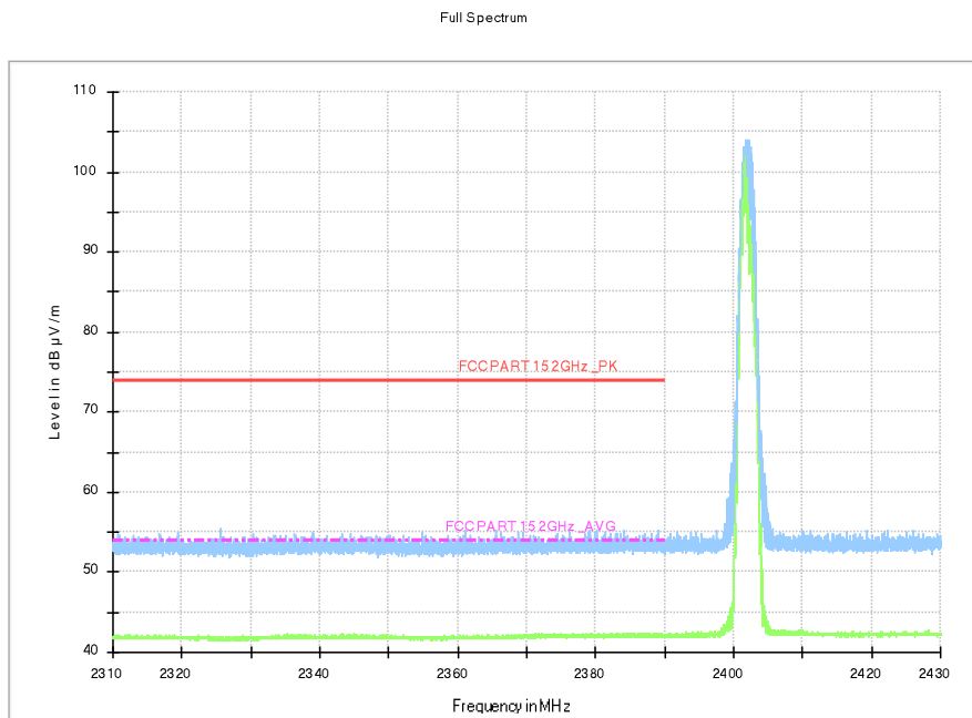
Fig.17. Frequency Band Edges: 8DPSK, Channel 0, 2.31 GHz - 2.43GHz
