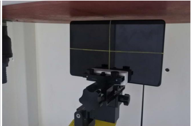
Edge 2 of EUT with Phantom 5 mm Gap
