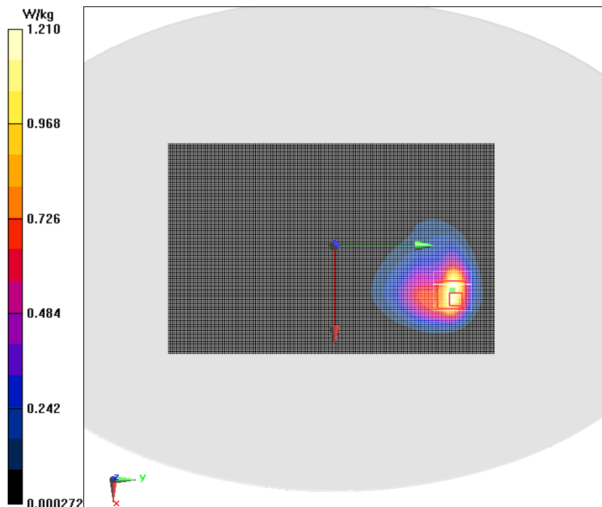
Fig.9 GSM1900 Ground Mode High 0mm With Headset
