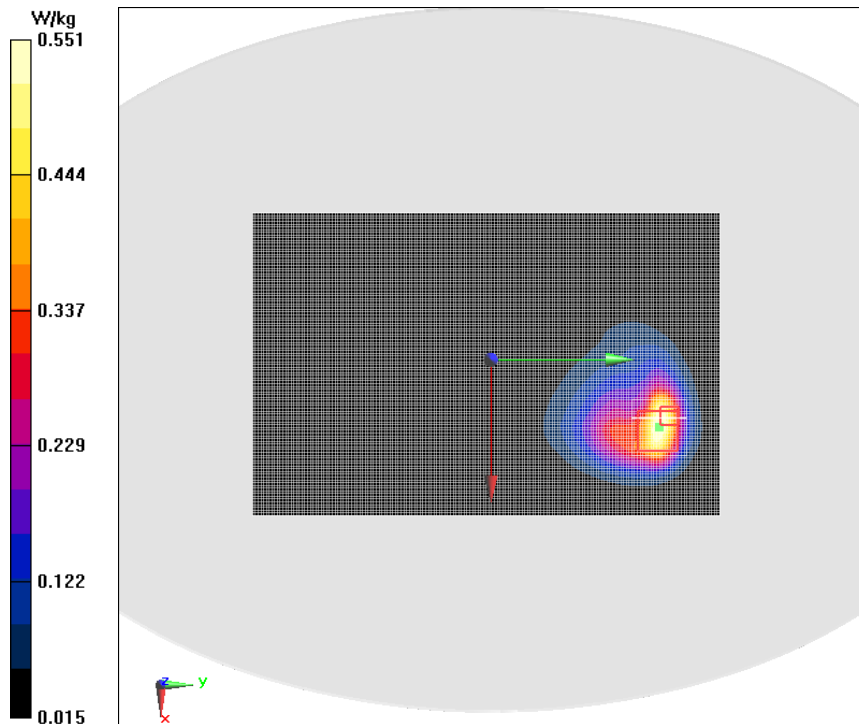
Fig.23 LTE Band 5 25RB 0offset Ground Mode Middle 0mm
