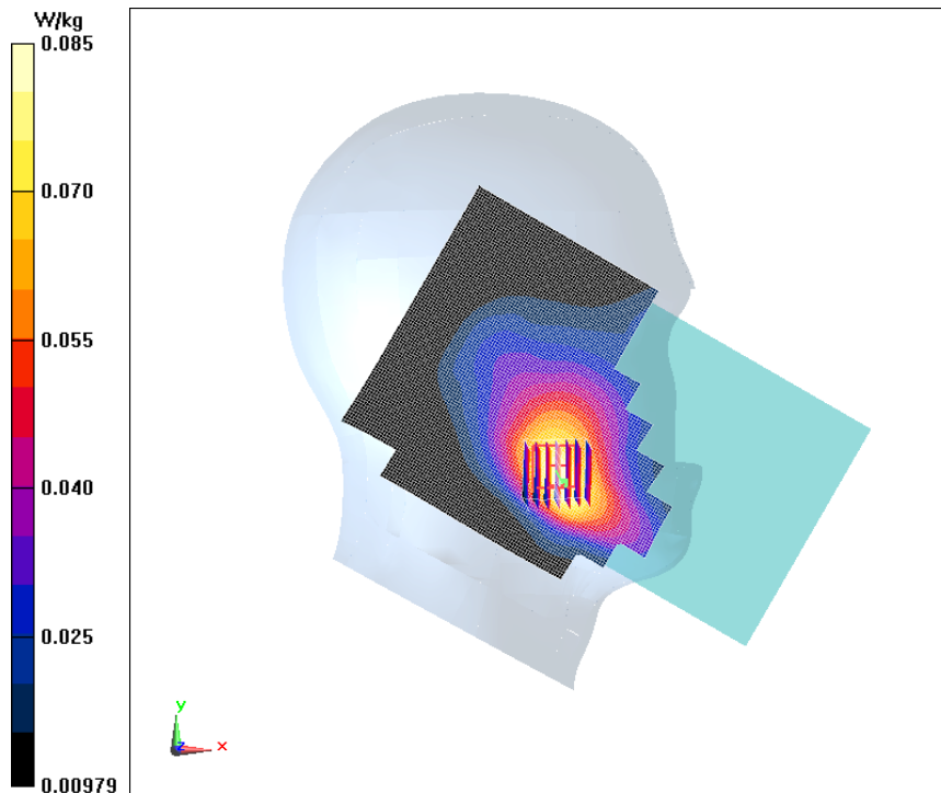
Fig.18 LTE Band 5 1RB 25 Offset Left Cheek Mode middle
