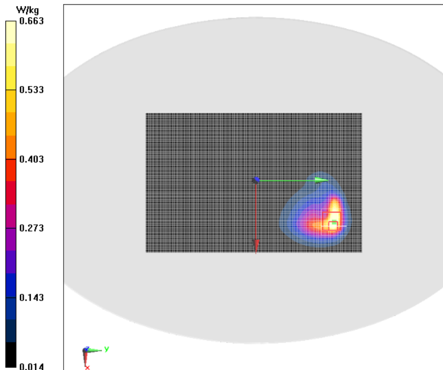
Fig.17 WCDMA Band 5 Ground Mode High 0mm
