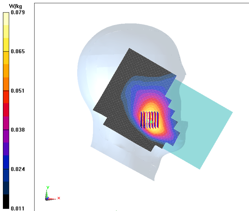
Fig.19 LTE Band 5 25RB 0 Offset Left Cheek Mode High
