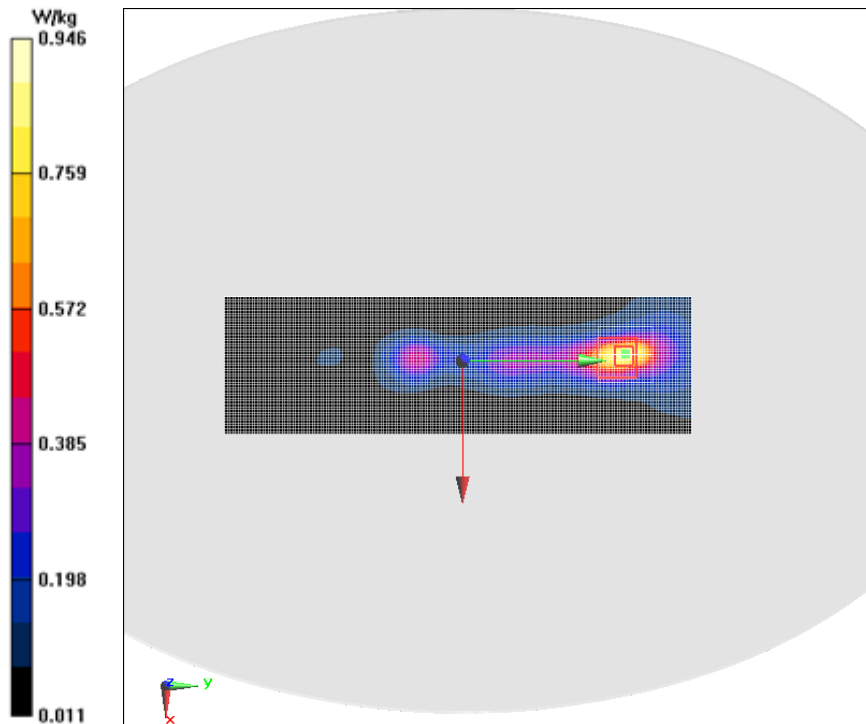
Fig.11 WCDMA Band 2 Right Mode High 0mm
