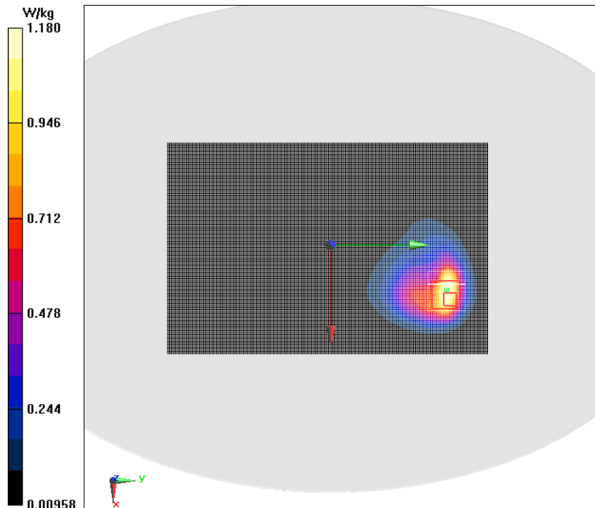
Fig.6 GSM1900 Ground Mode High 0mm
