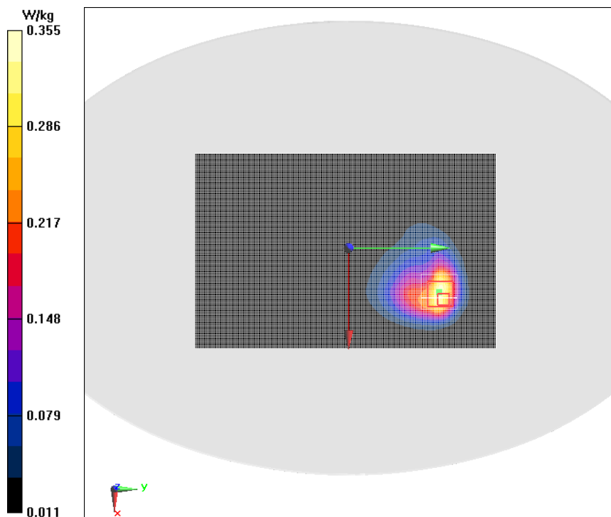
Fig.3 GSM850 4TS Ground Mode High 0mm
