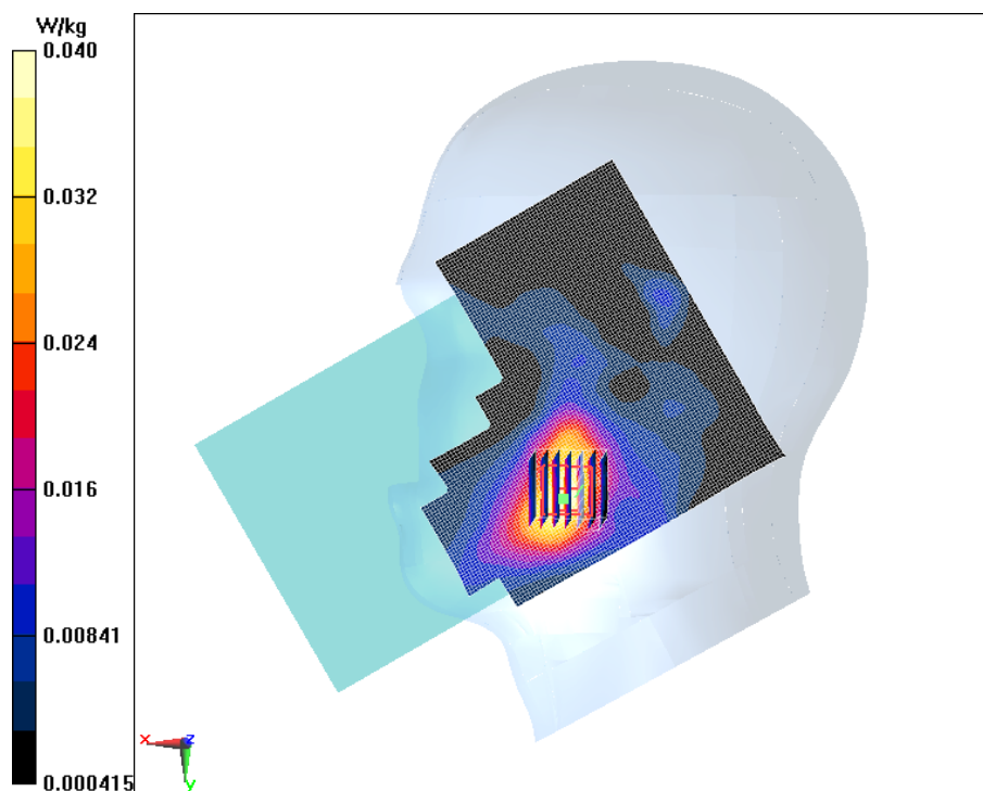
Fig.4 GSM1900 Right Cheek Mode High
