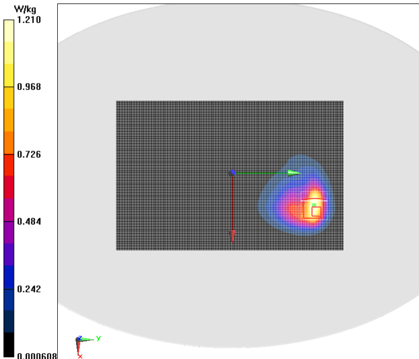
Fig.8 GSM1900 Ground Mode High 0mm SIM2
