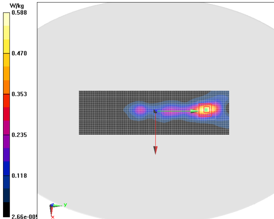
Fig.5 GSM1900 Right Mode High 0mm
