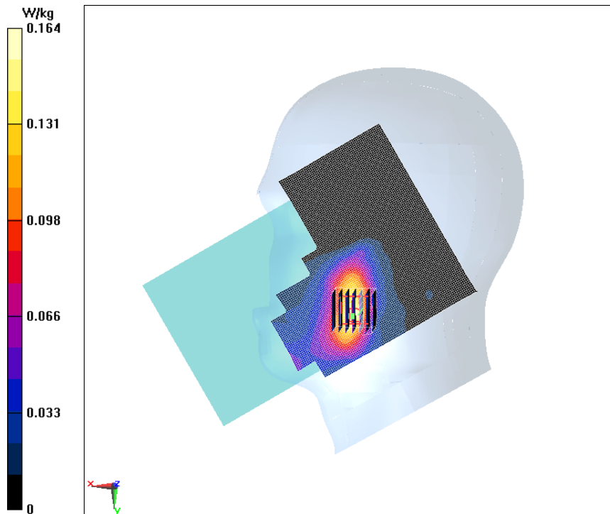
Fig.24 LTE Band 7 20MHz 1RB 50Offset Right Cheek Mode High
