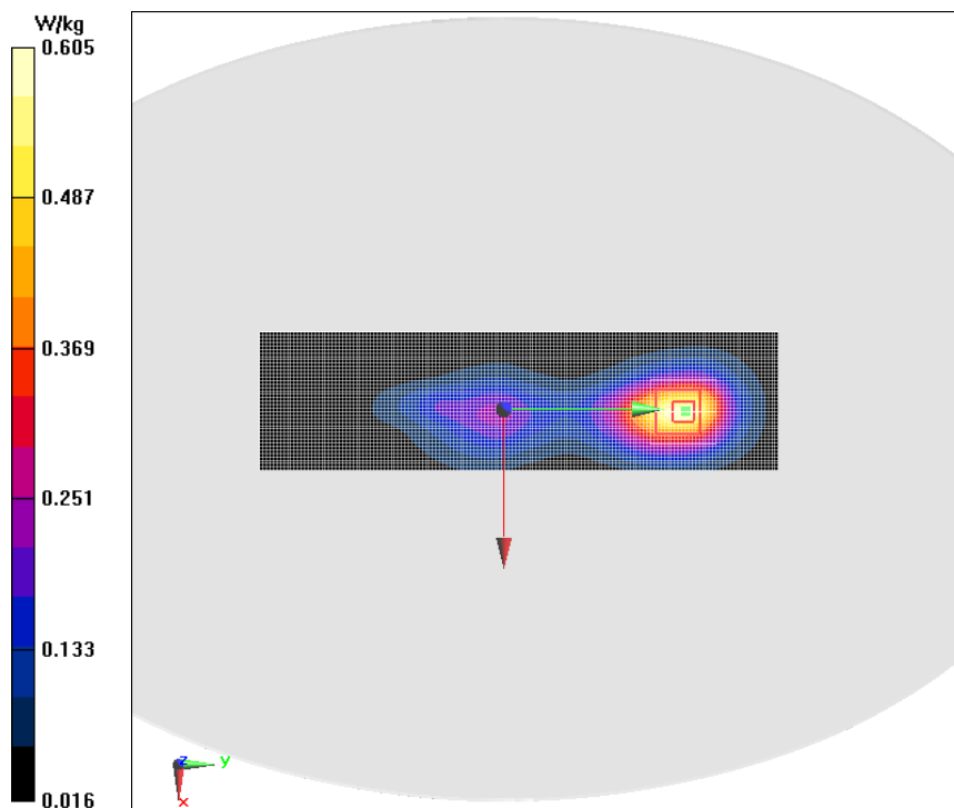
Fig.2 GSM850 4TS Right Mode High 0mm
