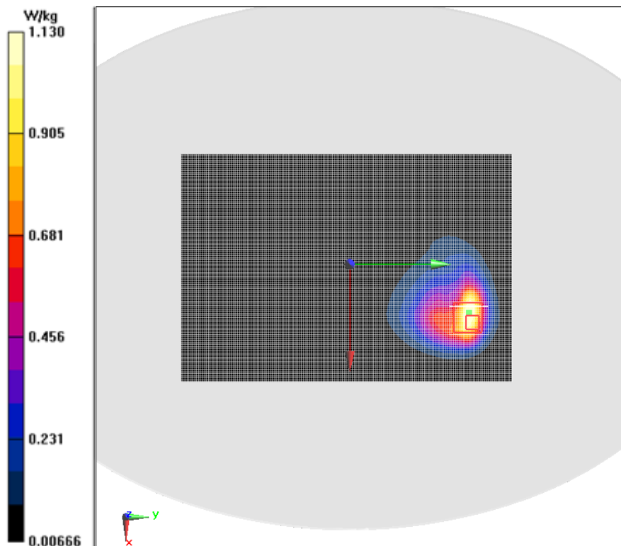
Fig.13 WCDMA Band 2 Ground Mode High 0mm
