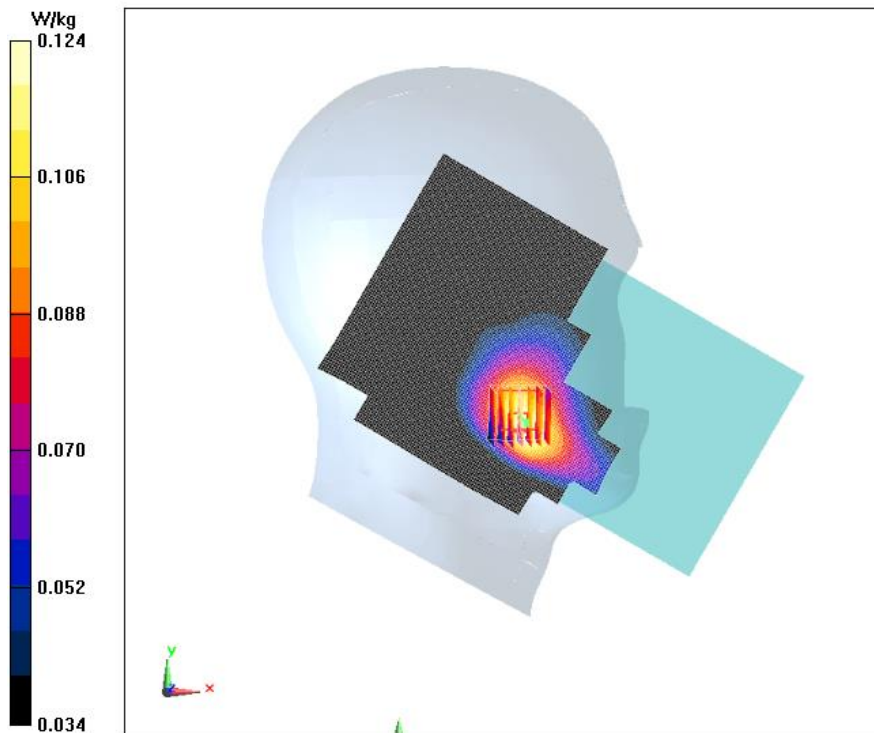
Fig.15 WCDMA Band 5 Left Cheek Mode High
