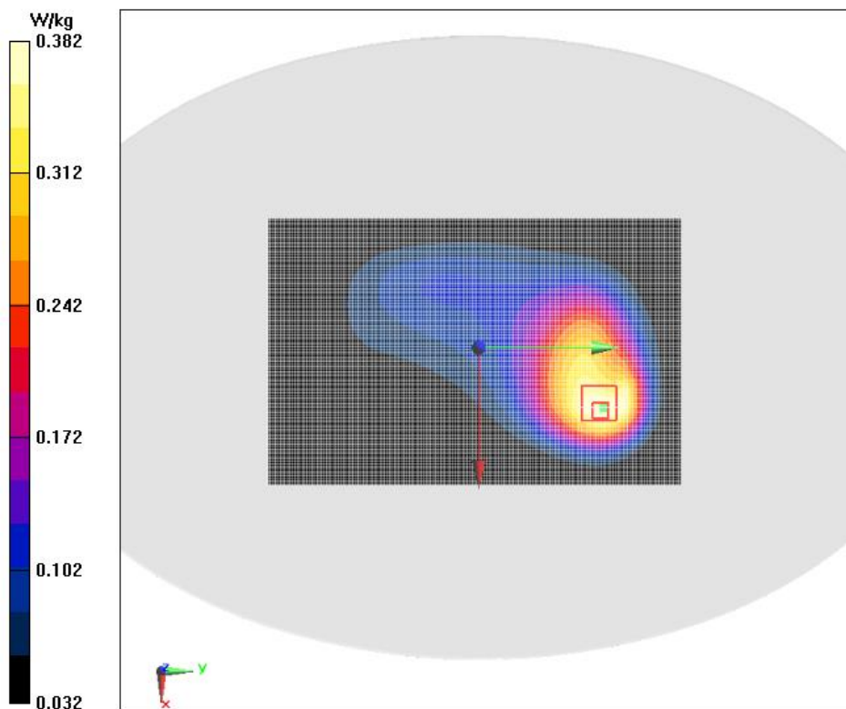
Fig.16 WCDMA Band 5 Ground Mode High 13mm
