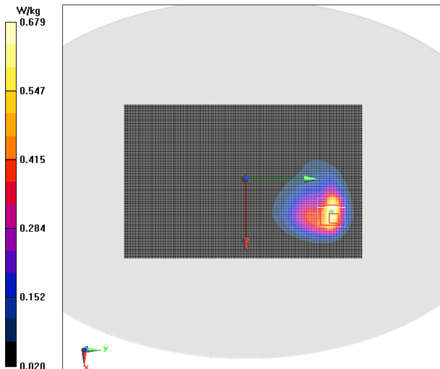
Fig.22 LTE Band 5 1RB 25 offset Ground Mode Low 0mm
