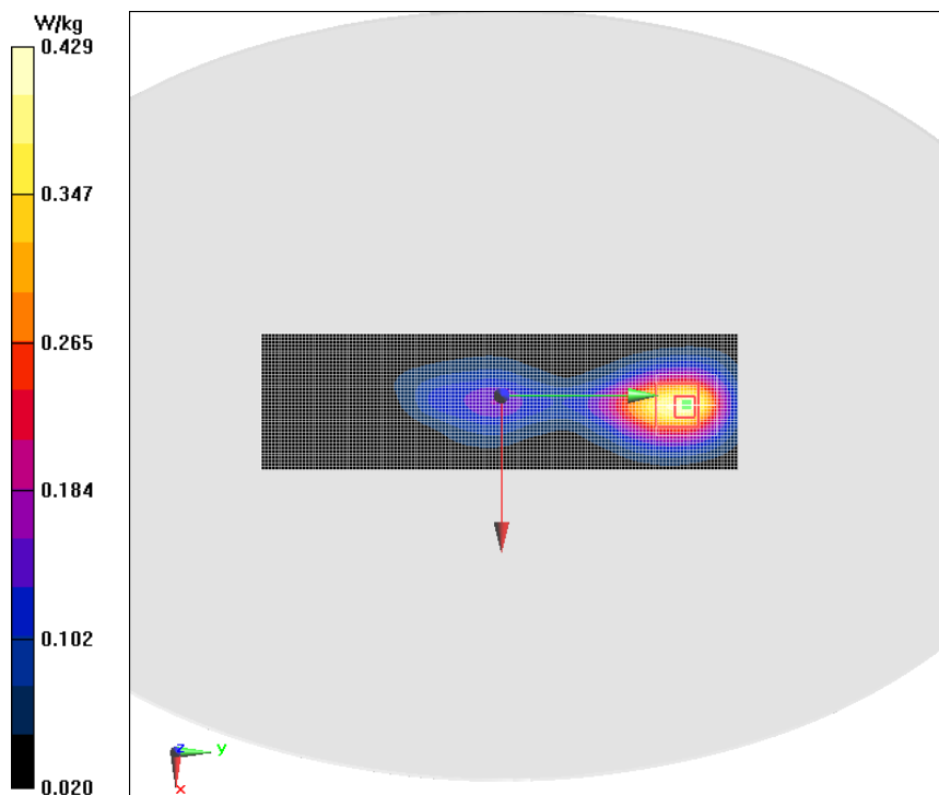
Fig.20 LTE Band 5 1RB 25 offset Right Mode High 0mm
