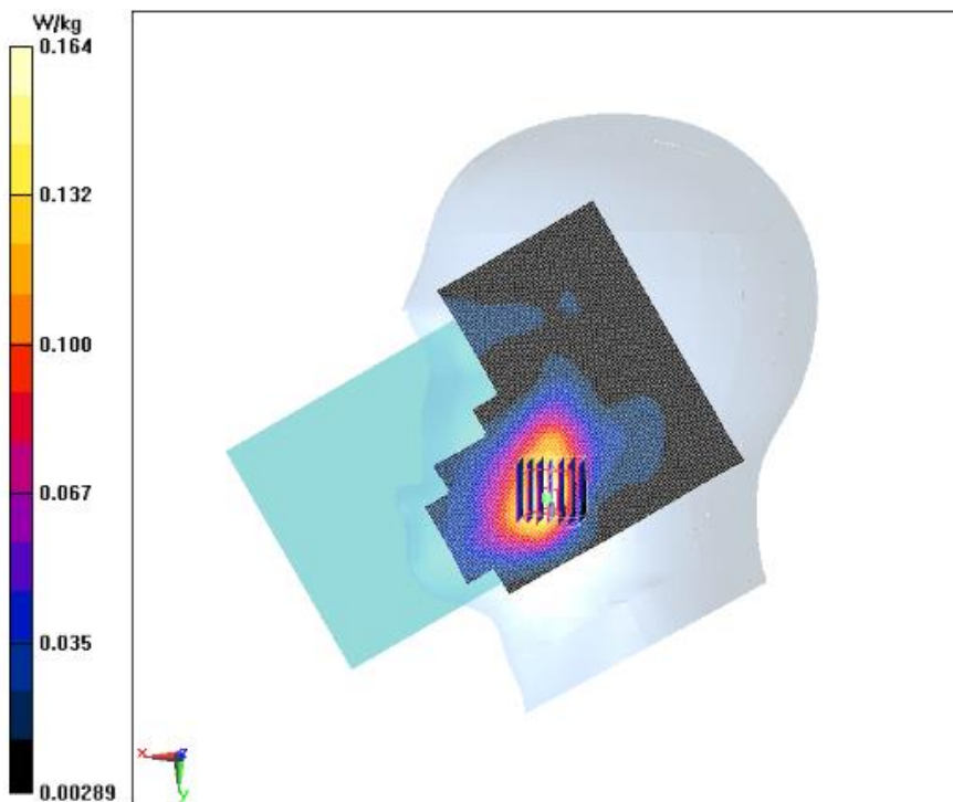
Fig.10 WCDMA Band 2 Right Cheek Mode High
