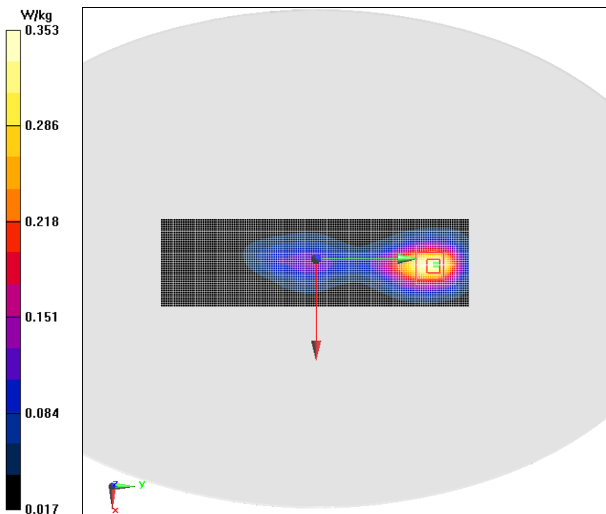
Fig.21 LTE Band 5 25RB 0 offset Right Mode High 0mm
