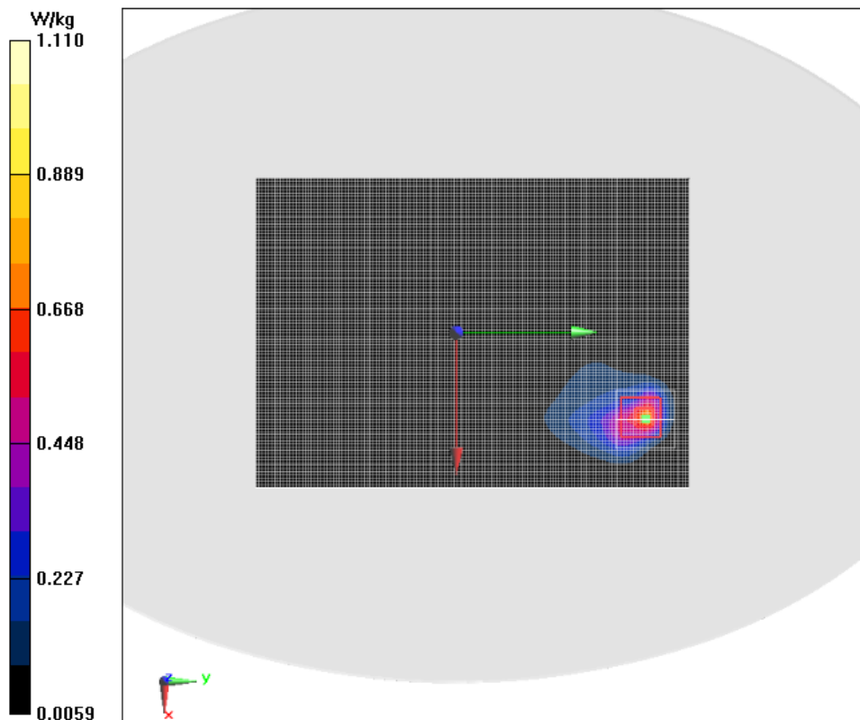
Fig.14 WCDMA Band 2 Ground Mode High 0mm Repeated
