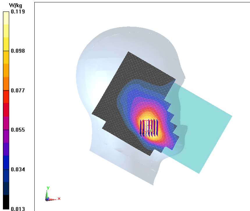
Fig.1 GSM900 Left Cheek Mode High
