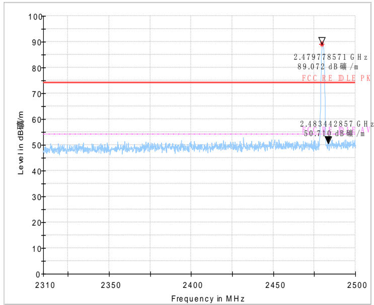
Bandedge:ch39
