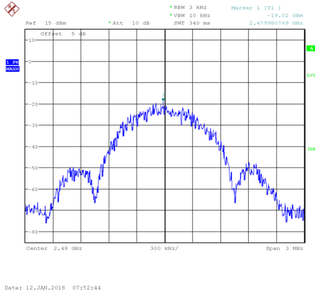
Fig.6 Power spectral density: CH39
