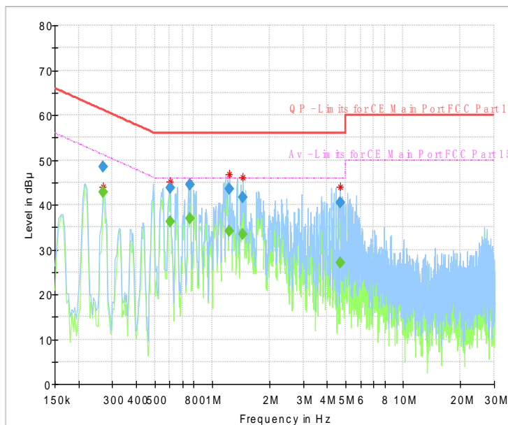
Fig.24 AC Powerline Conducted Emission
