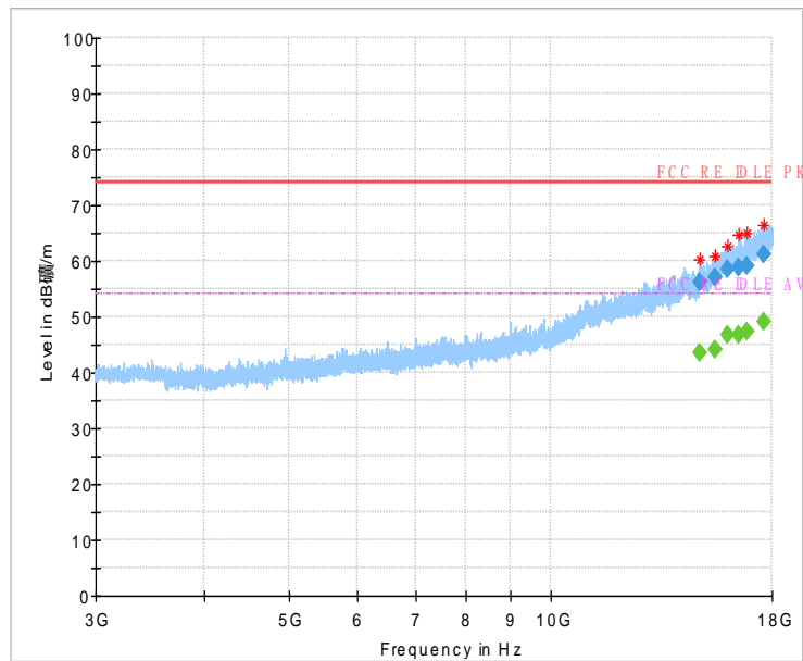
Fig.57 Radiated Spurious Emission (802.11 n-20MHz,Ch1,3GHz~18GHz)
