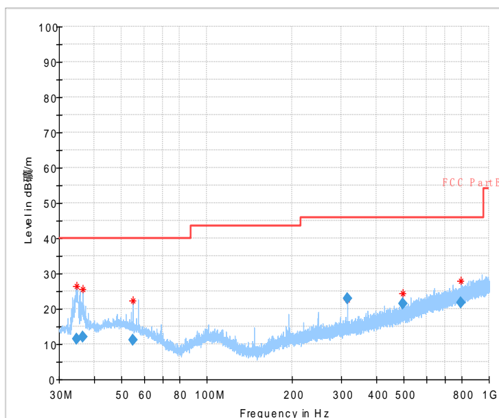
Fig.55 Radiated Spurious Emission (802.11 n-20MHz,Ch1,30MHz~1GHz)
