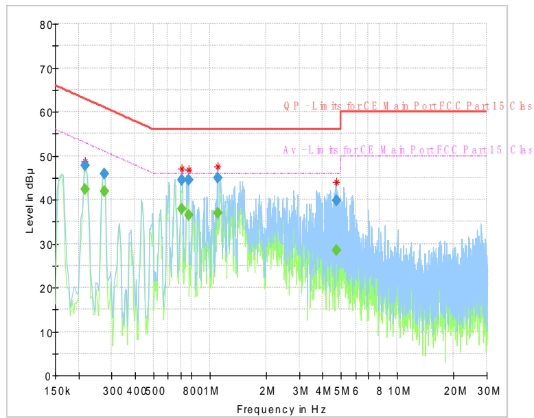
Fig.58 AC Powerline Conducted Emission
