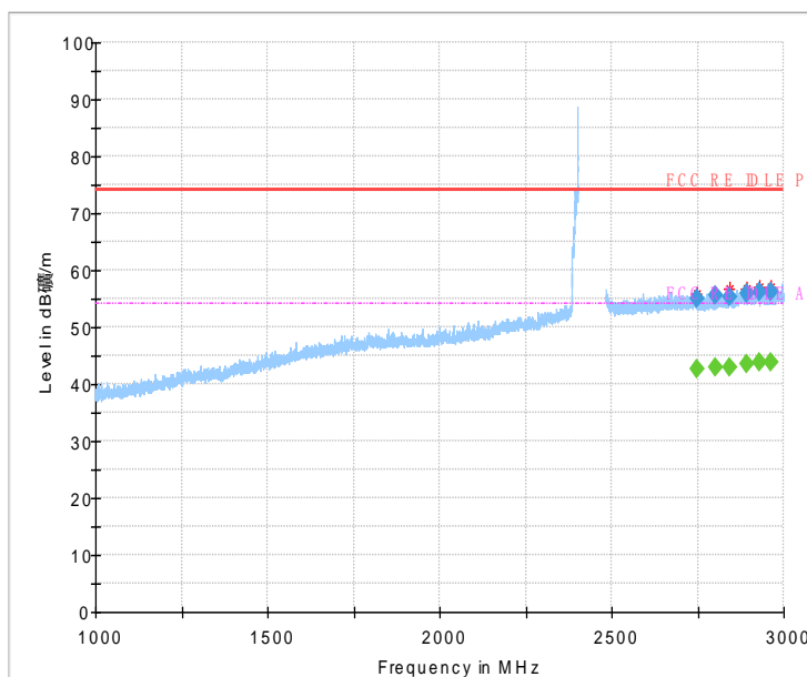
Fig.56 Radiated Spurious Emission (802.11 n-20MHz,Ch1,1GHz~3GHz)
