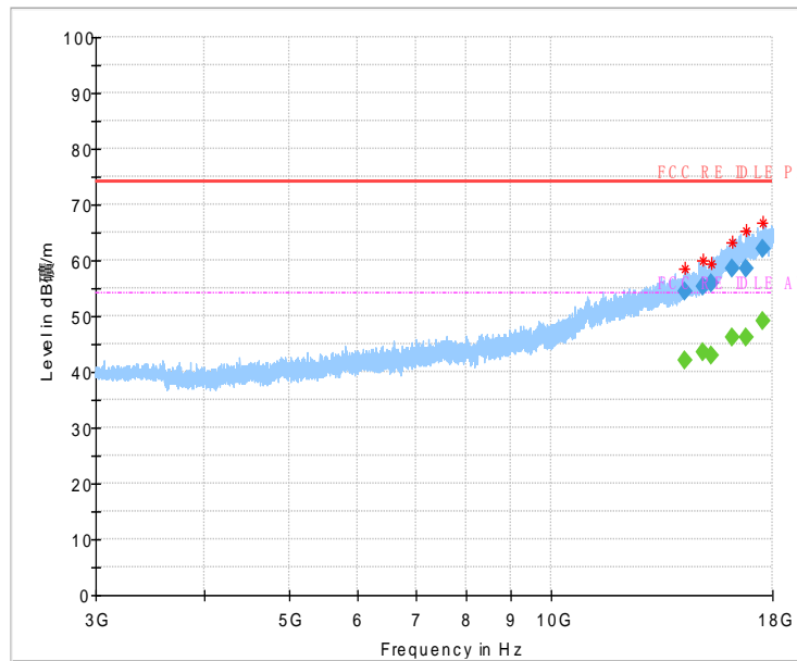
Fig.52 Radiated Spurious Emission (802.11g,Ch1,3GHz~18GHz)
