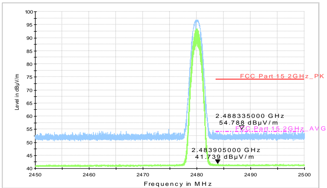
RE-BT-Power_2.45G-2.5GHz
