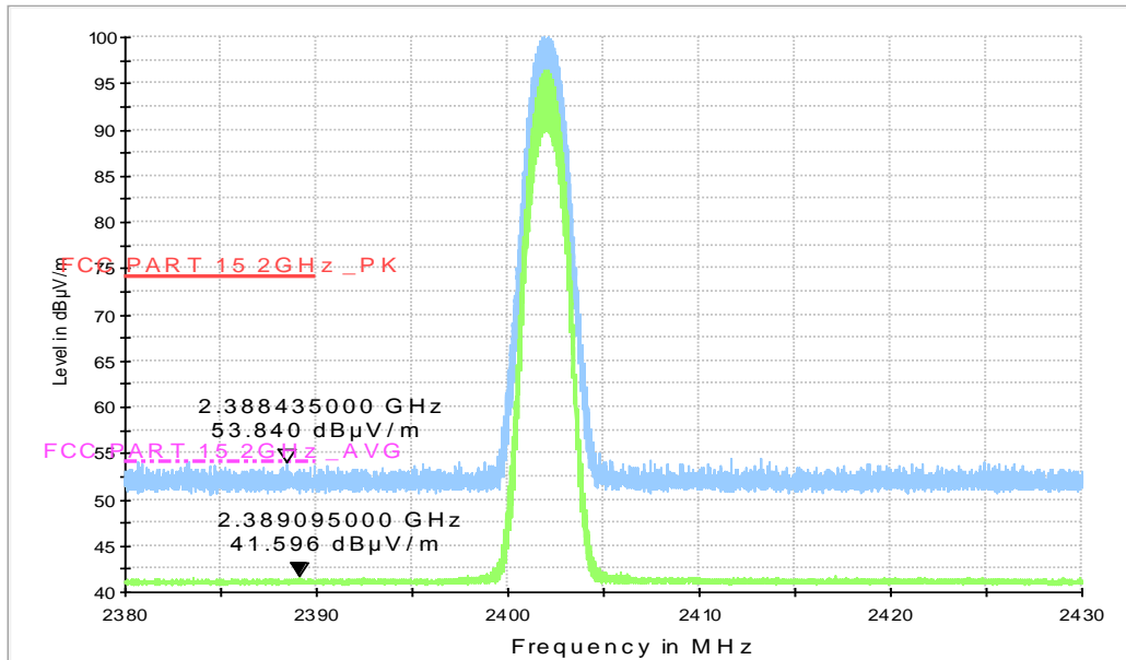
RE-BT-Power_2.38G-2.43GHz
