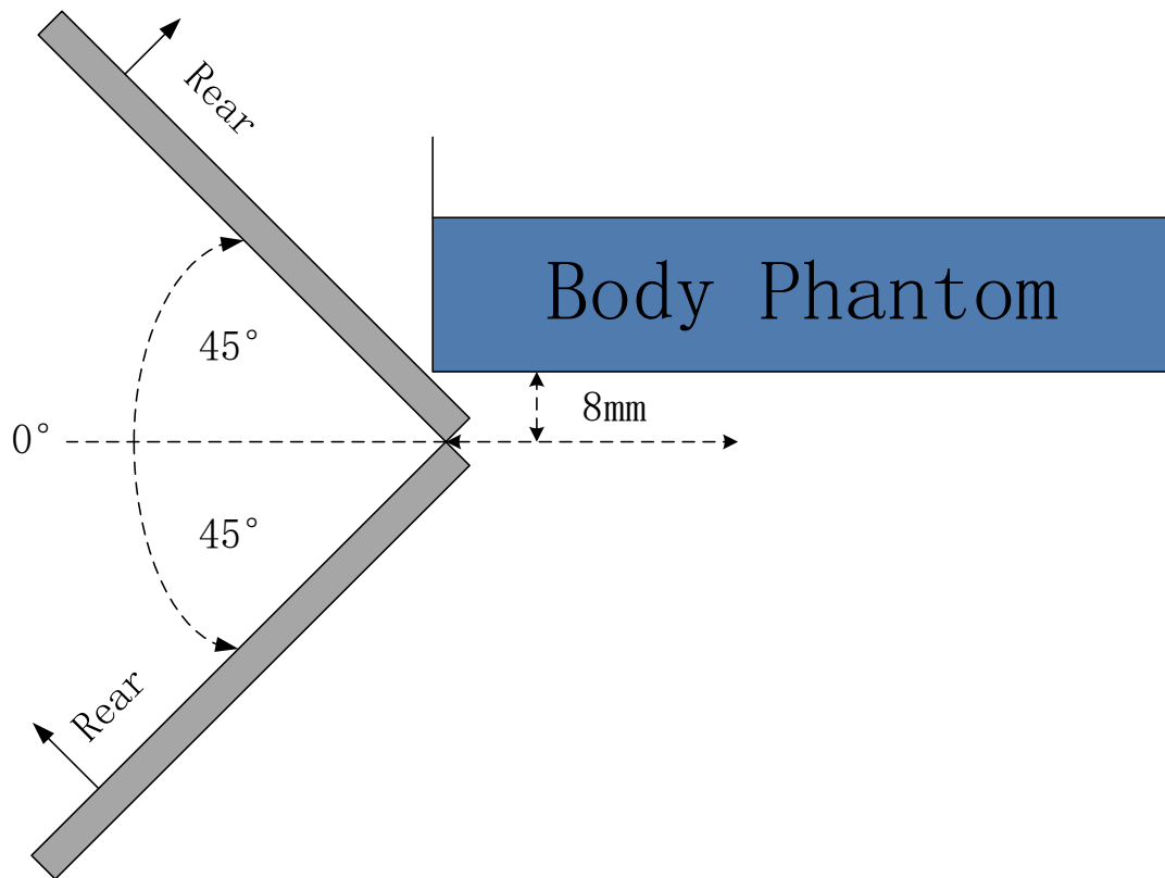
The rear evaluation for WiFi antenna
