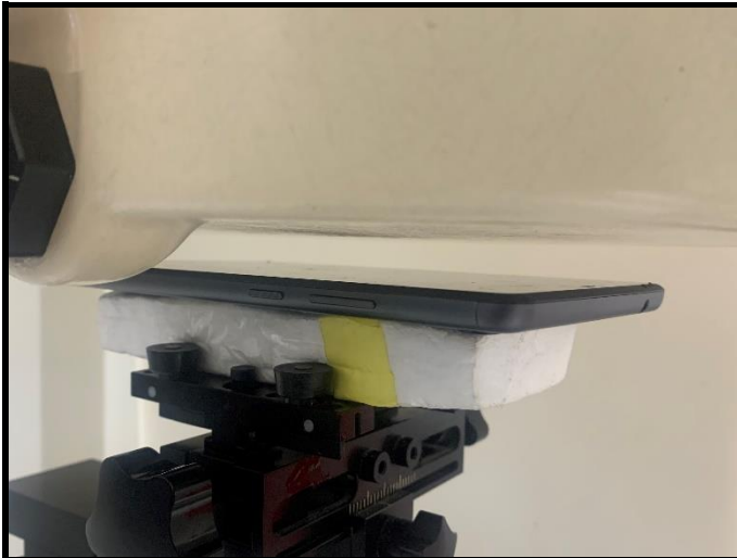
Front Face of EUT with 1.3 cm Gap
