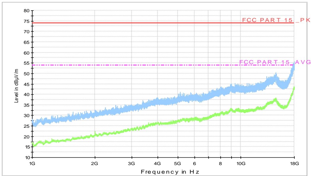
Normal RE_1G-18GHz_directly
